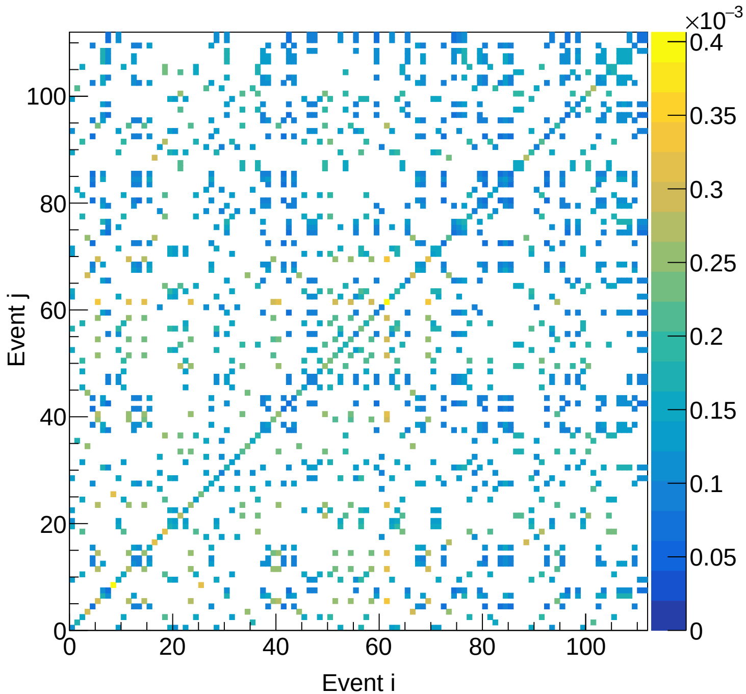
LD2 (total) Covariance | M: [5.7, 6.0] xF: [0.25, 0.30)
