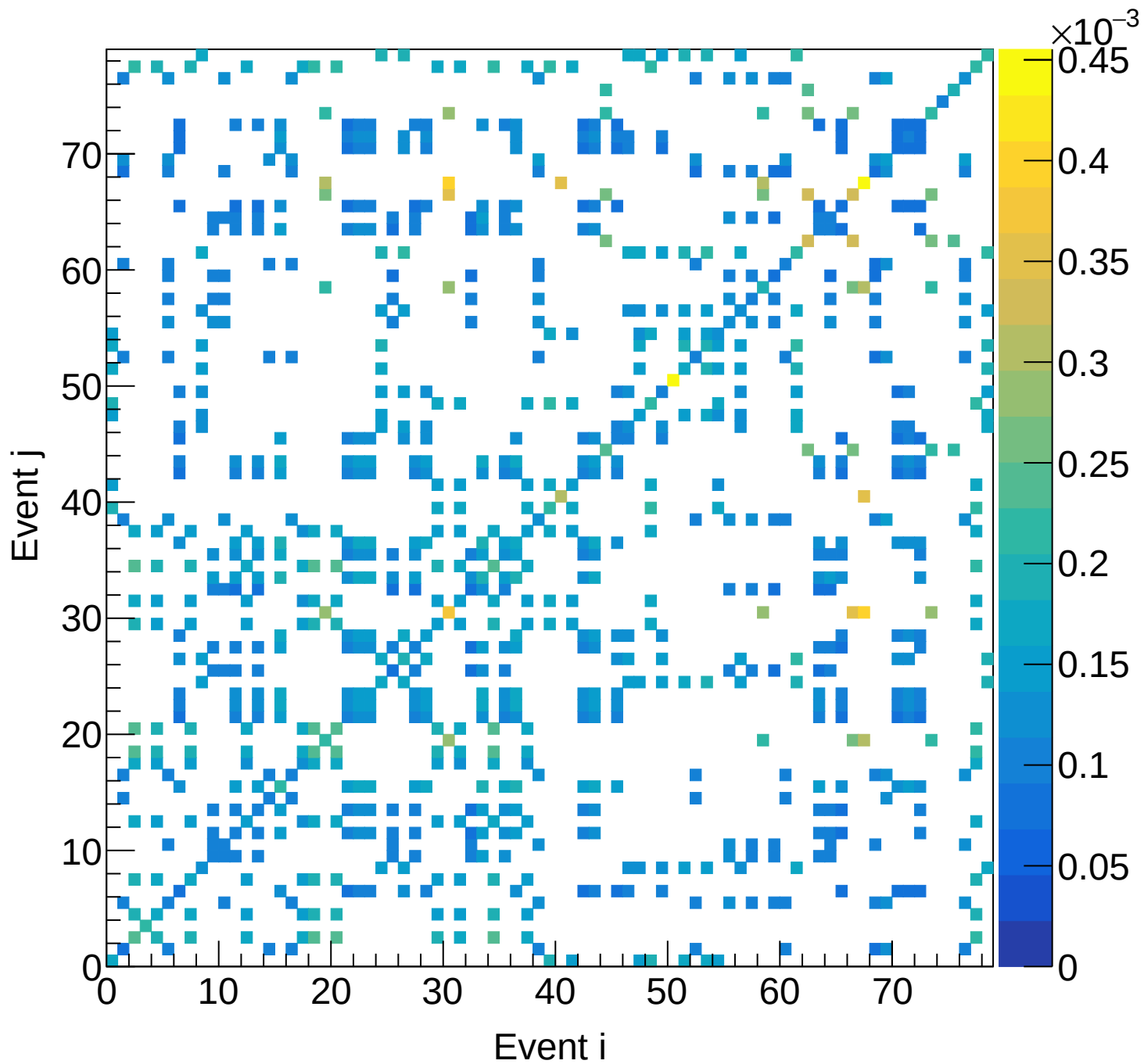
LD2 (total) Covariance | M: [6.0, 6.3) xF: [0.25, 0.30)
