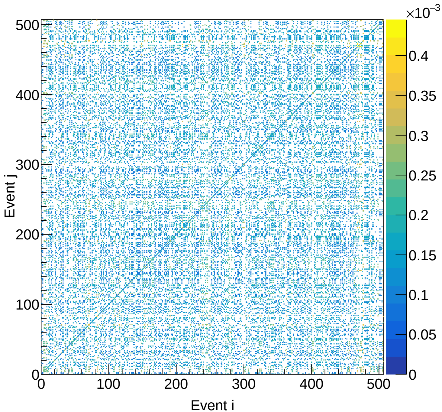
LD2 (total) Covariance | M: [3.9, 4.2) xF: [0.30, 0.35)
