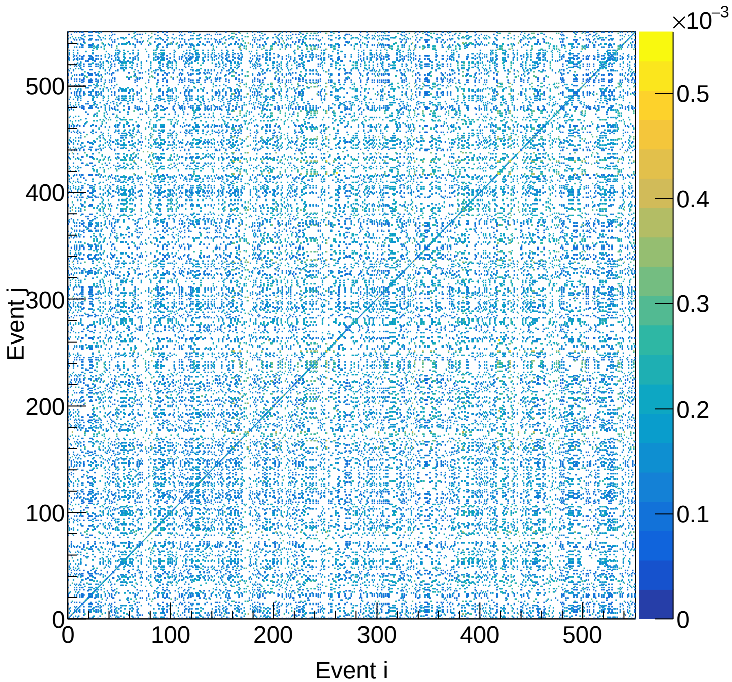
LD2 (total) Covariance | M: [4.2, 4.5) xF: [0.30, 0.35)
