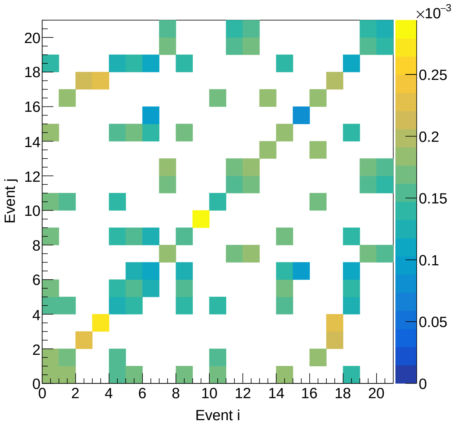
LD2 (total) Covariance | M: [6.9, 7.5) xF: [0.30, 0.35)
