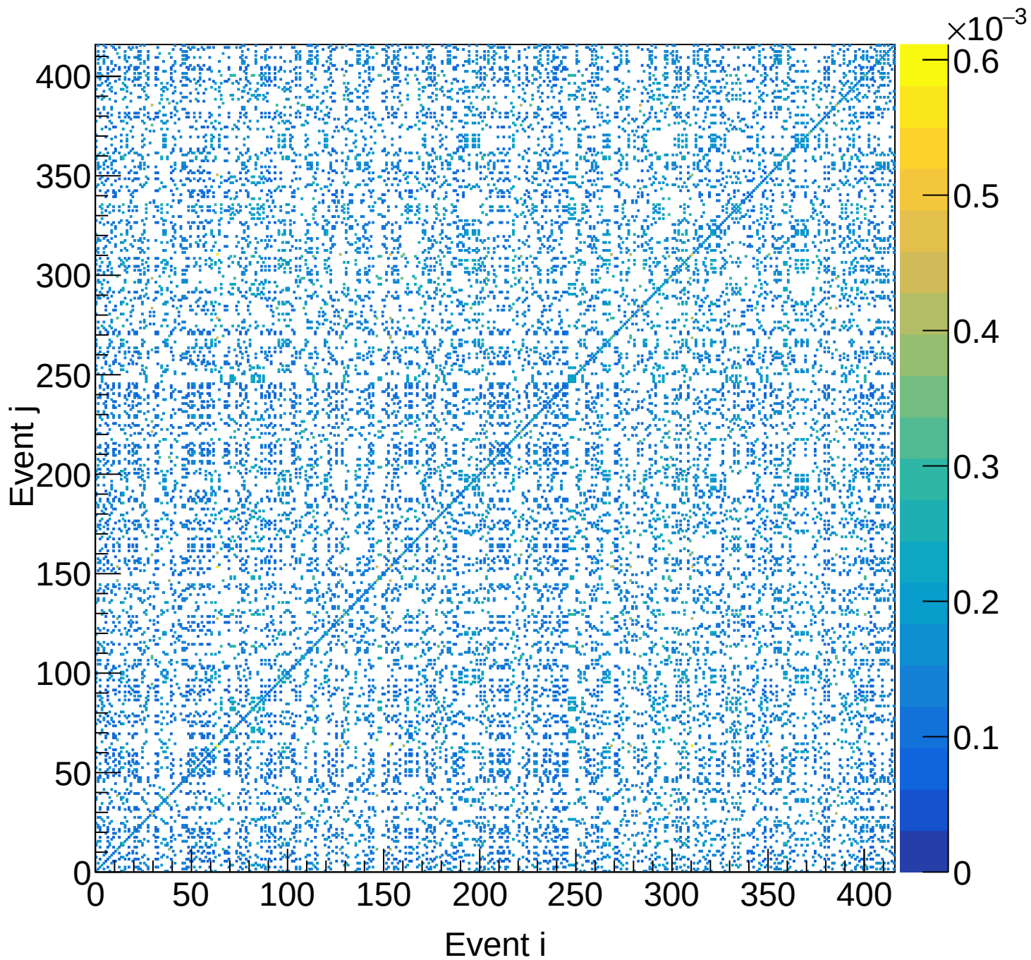
LD2 (total) Covariance | M: [4.8, 5.1) xF: [0.30, 0.35)
