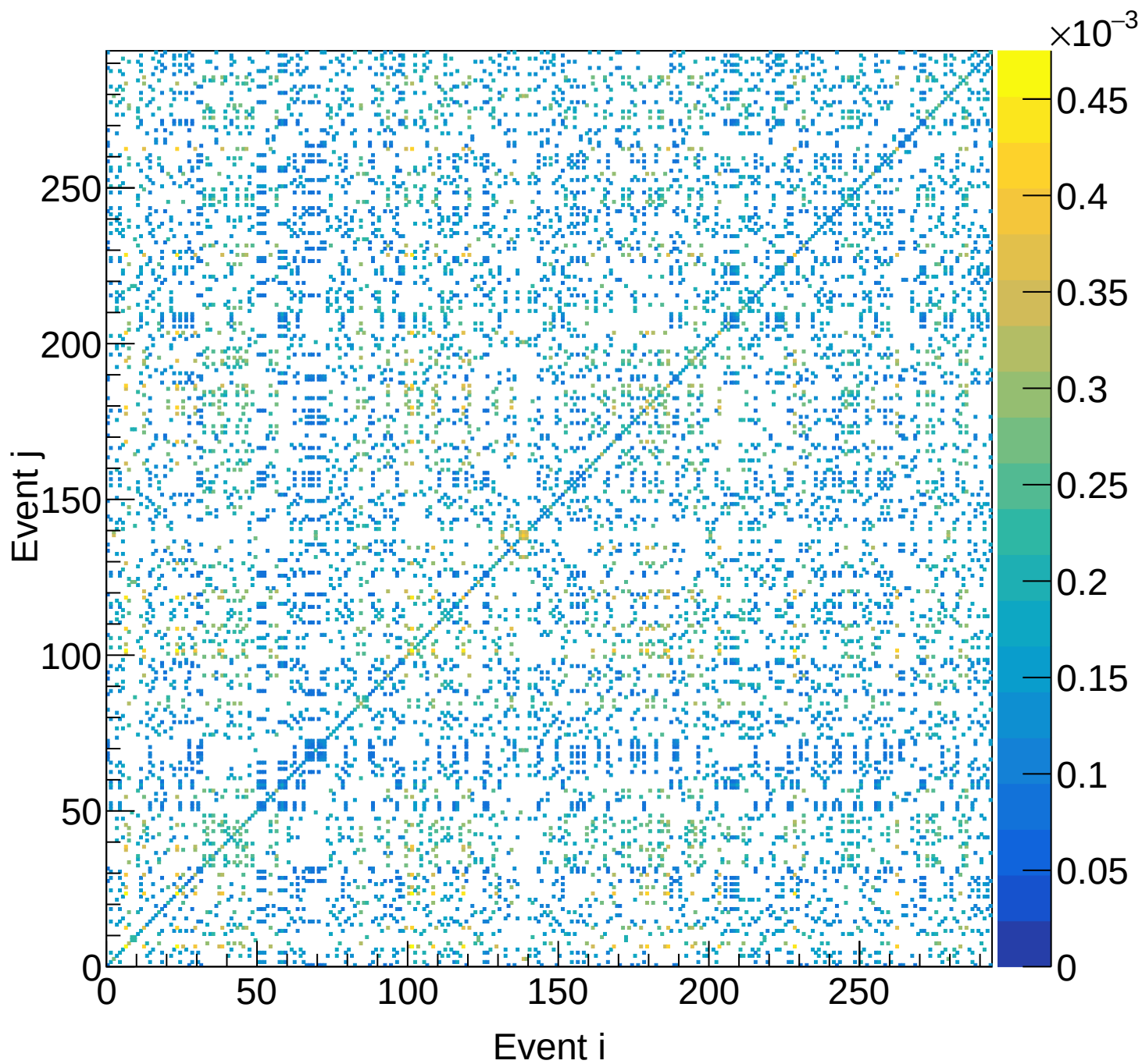
LD2 (total) Covariance | M: [5.1, 5.4) xF: [0.30, 0.35)
