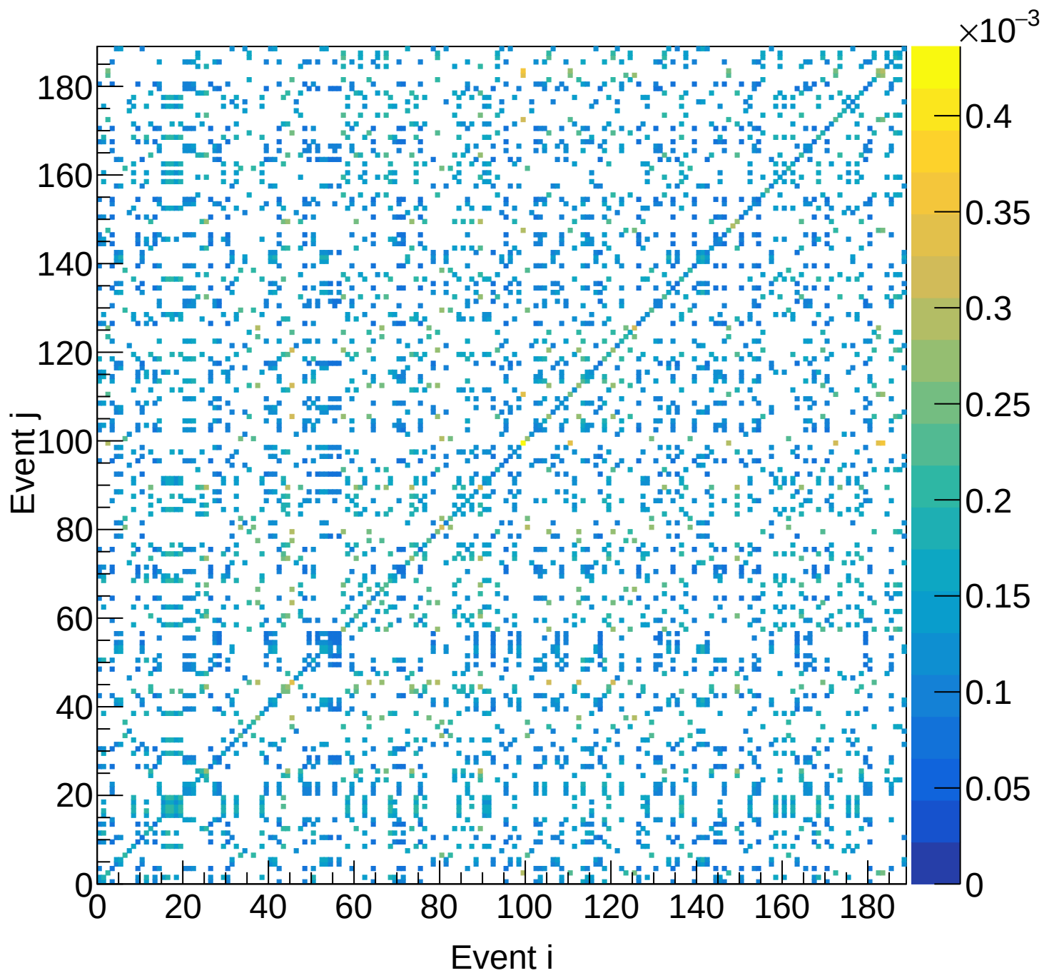
LD2 (total) Covariance | M: [5.4, 5.7) xF: [0.30, 0.35)
