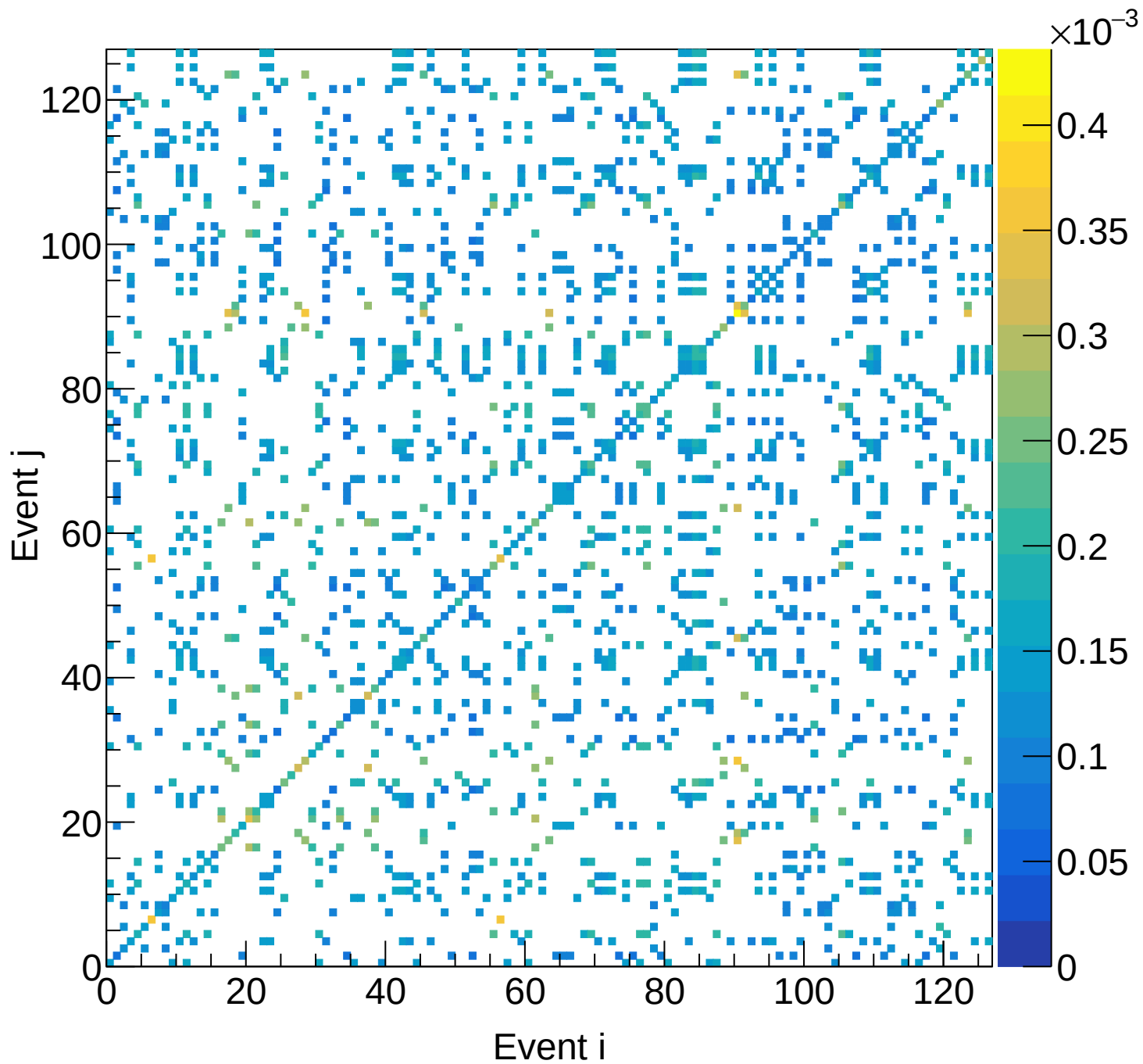
LD2 (total) Covariance | M: [5.7, 6.0) xF: [0.30, 0.35)
