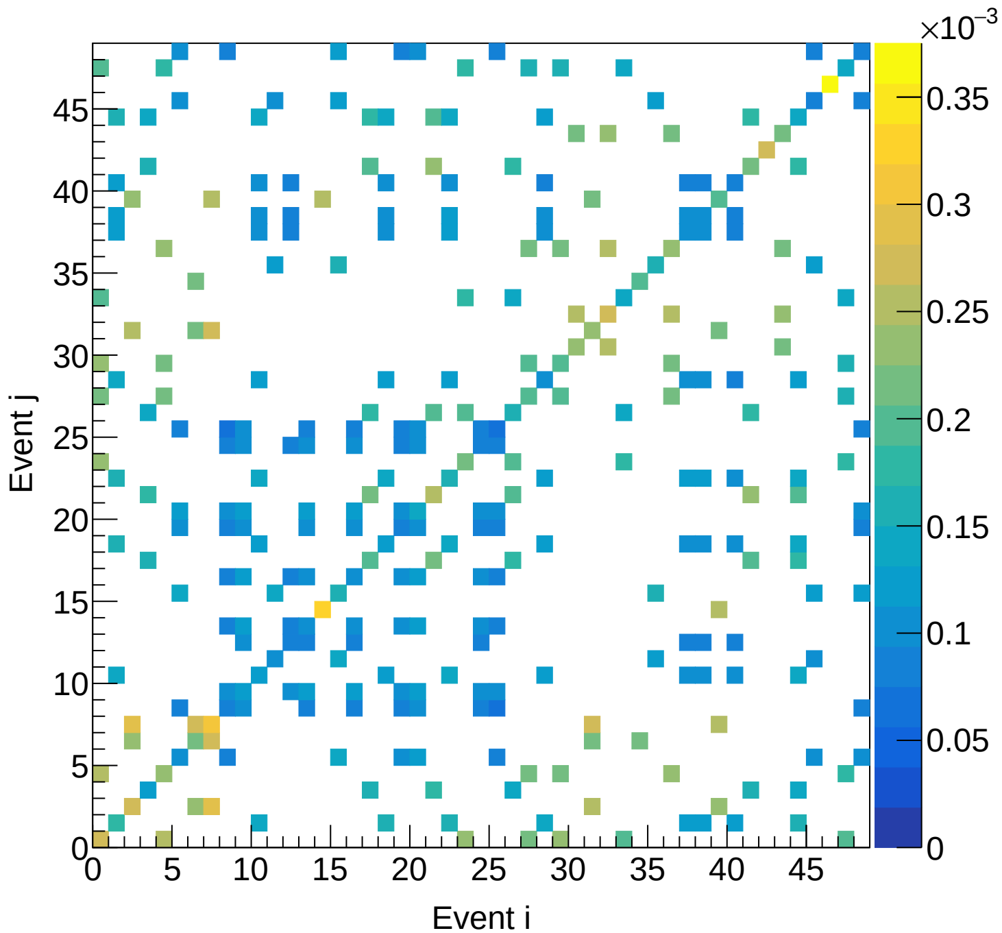
LD2 (total) Covariance | M: [6.3, 6.6) xF: [0.30, 0.35)
