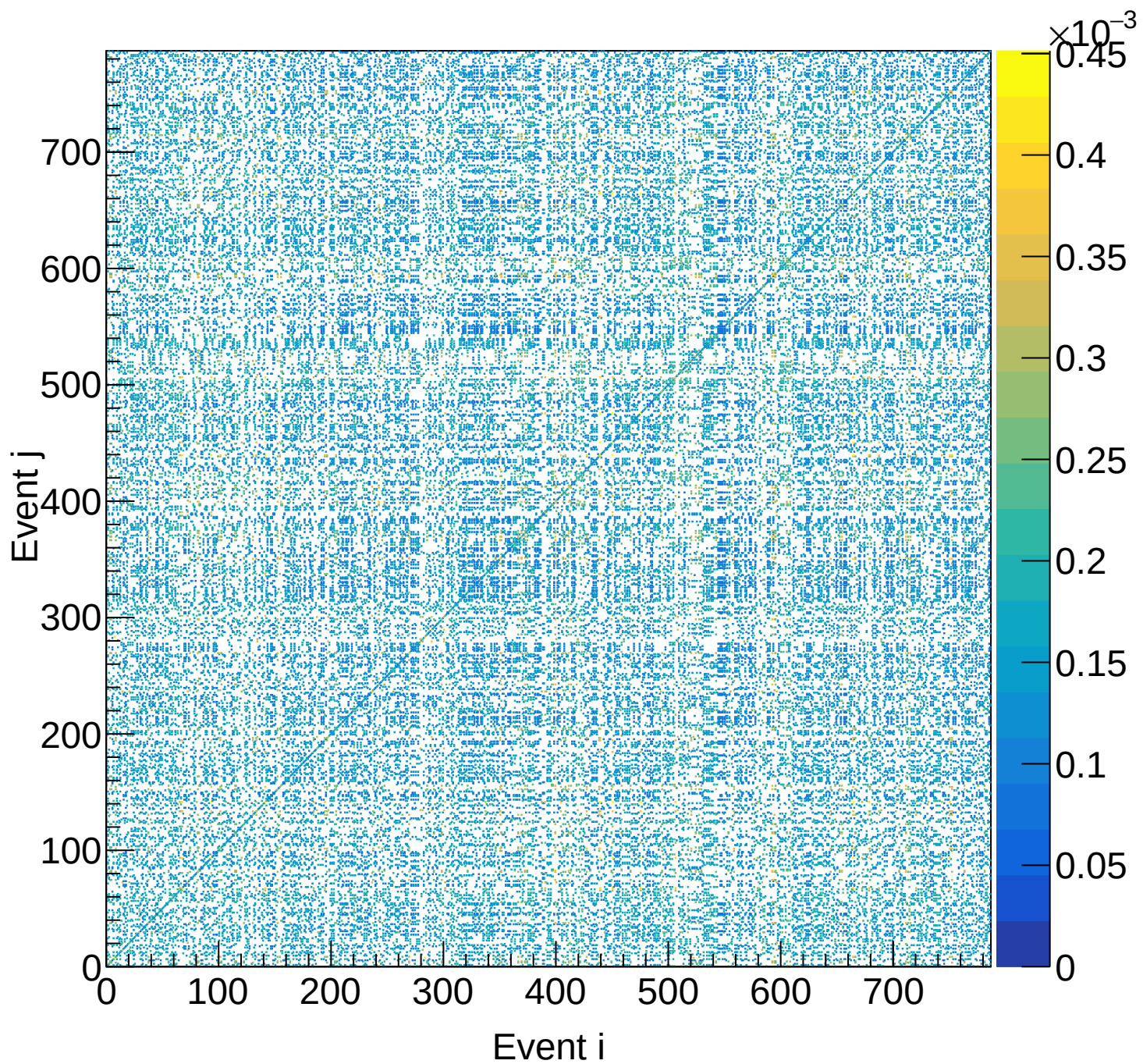
LD2 (total) Covariance | M: [3.9, 4.2) xF: [0.35, 0.40)
