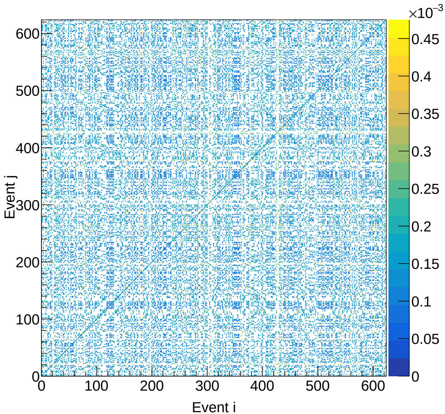
LD2 (total) Covariance | M: [4.2, 4.5) xF: [0.35, 0.40)
