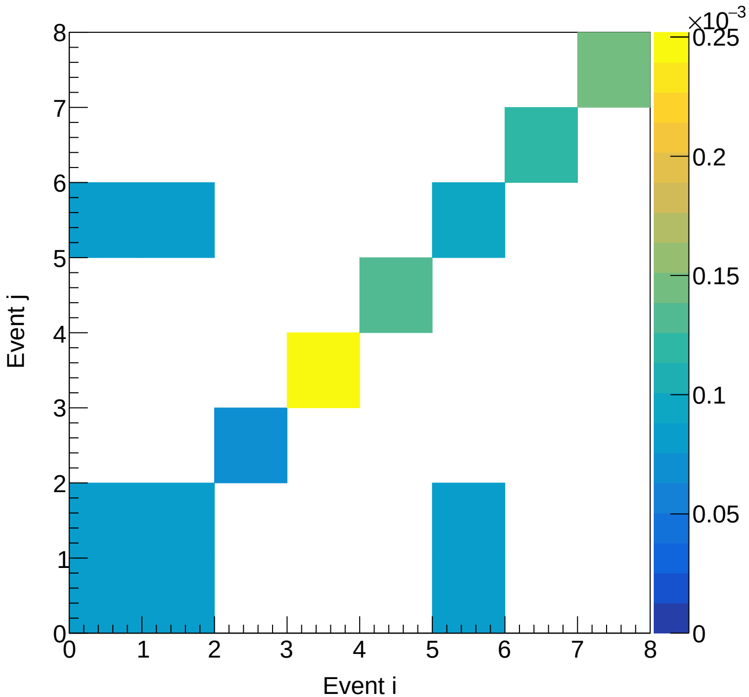
LD2 (total) Covariance | M: [7.5, 8.8) xF: [0.35, 0.40)
