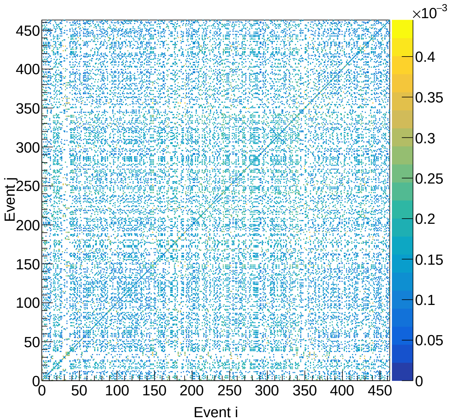
LD2 (total) Covariance | M: [4.8, 5.1) xF: [0.35, 0.40)
