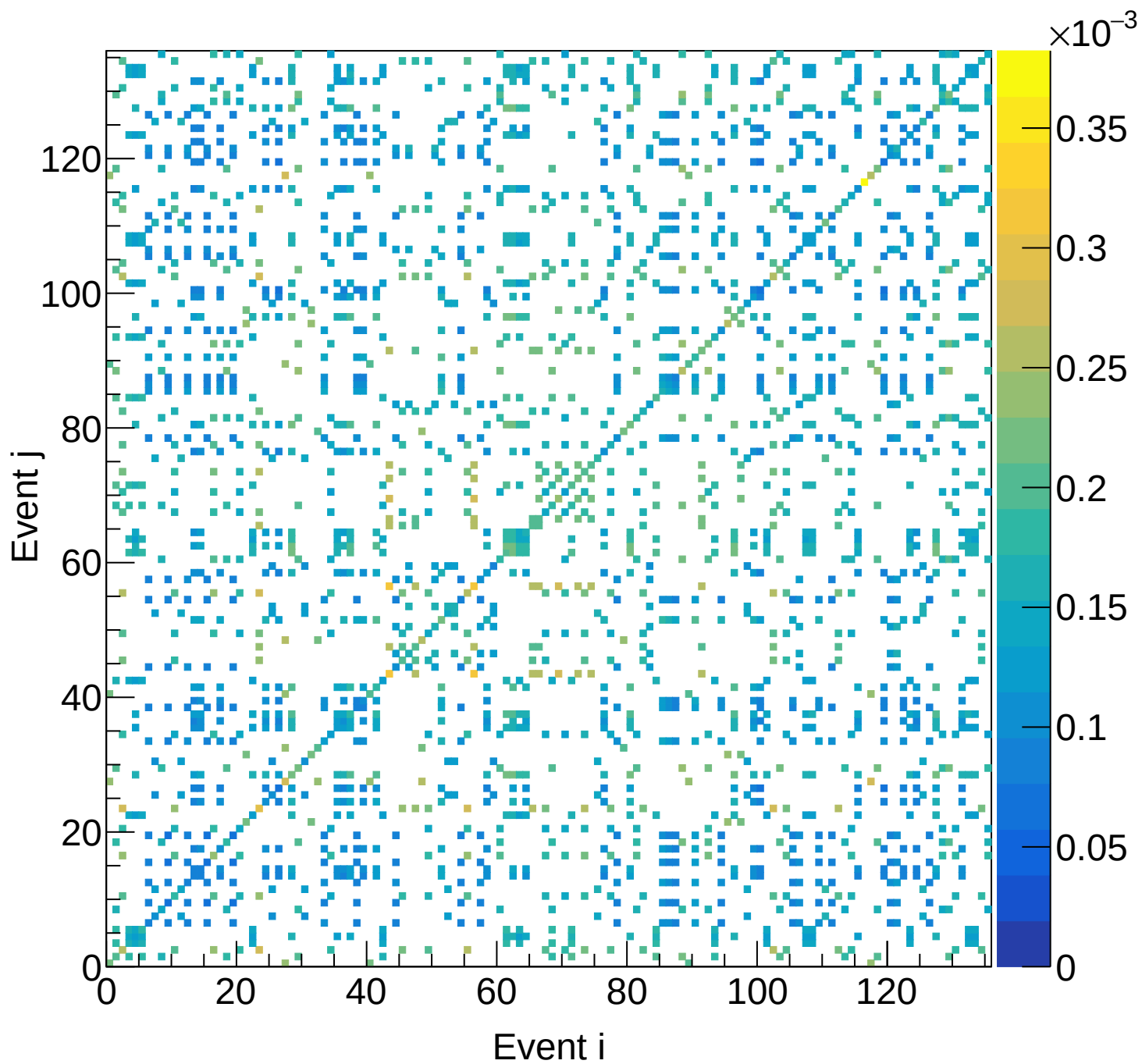
LD2 (total) Covariance | M: [5.7, 6.0] xF: [0.35, 0.40)
