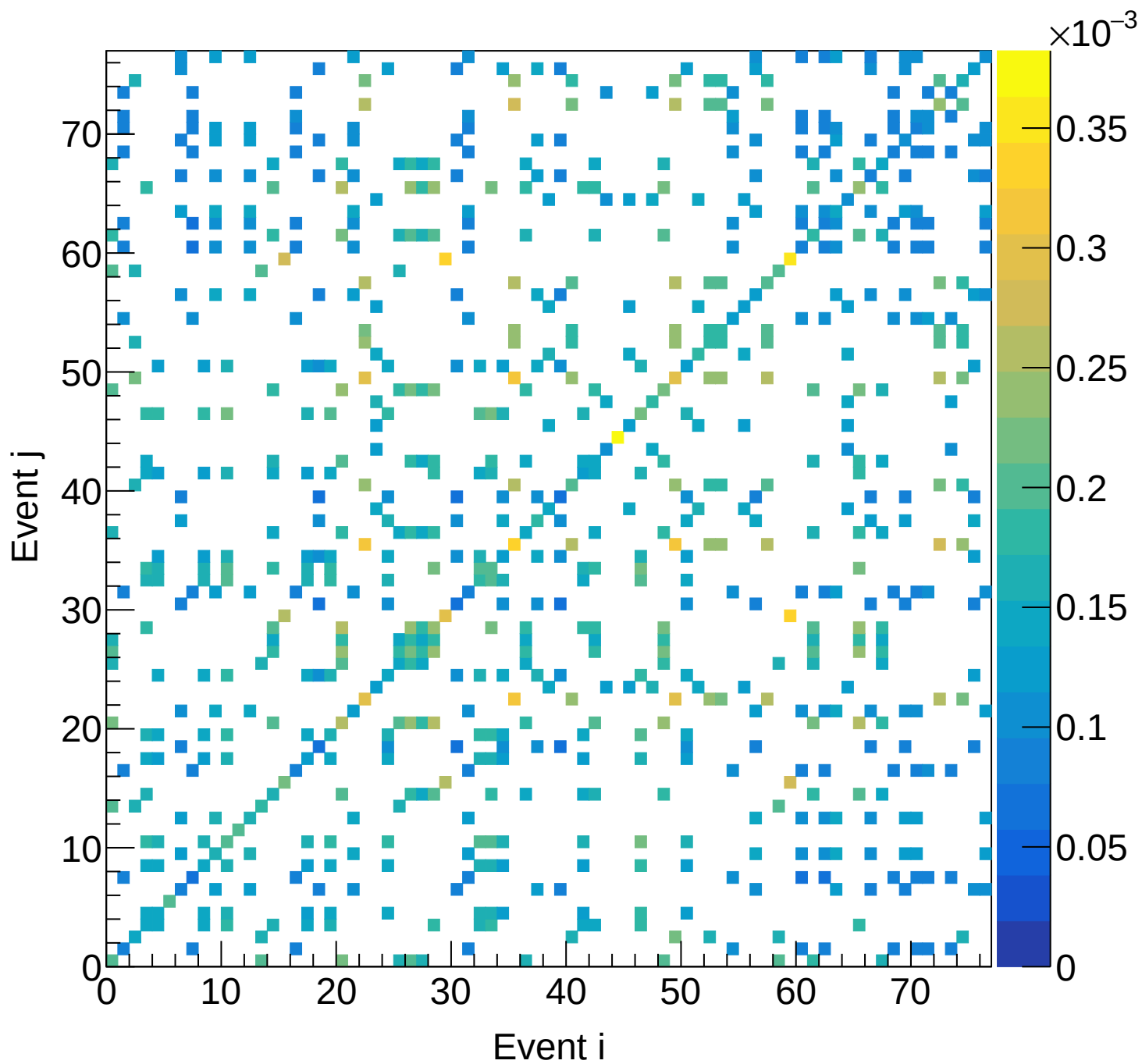
LD2 (total) Covariance | M: [6.0, 6.3) xF: [0.35, 0.40)
