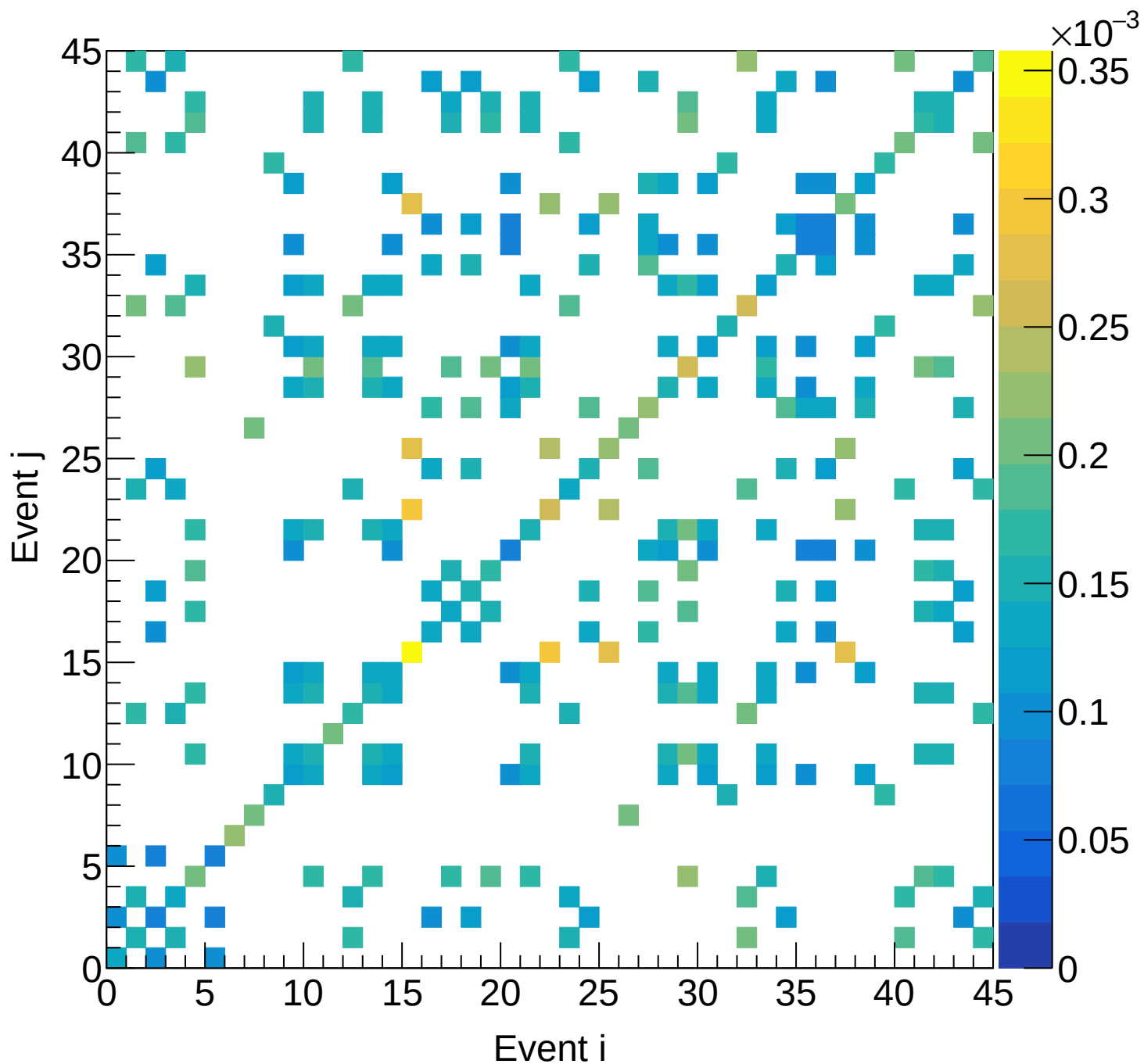
LD2 (total) Covariance | M: [6.3, 6.6] xF: [0.35, 0.40]
