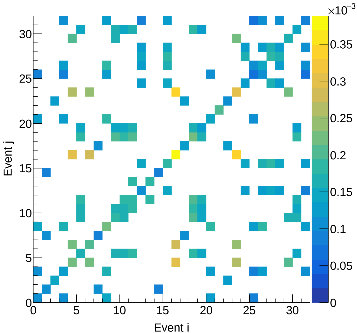
LD2 (total) Covariance | M: [6.6, 6.9] xF: [0.35, 0.40)
