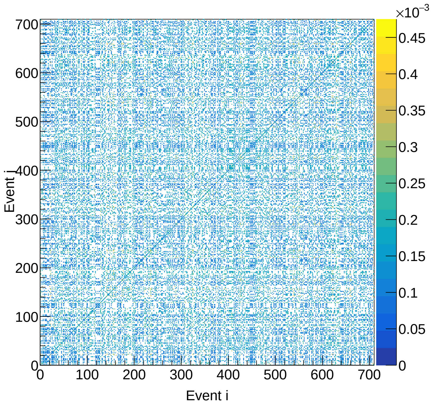
LD2 (total) Covariance | M: [4.2, 4.5) xF: [0.40, 0.45)
