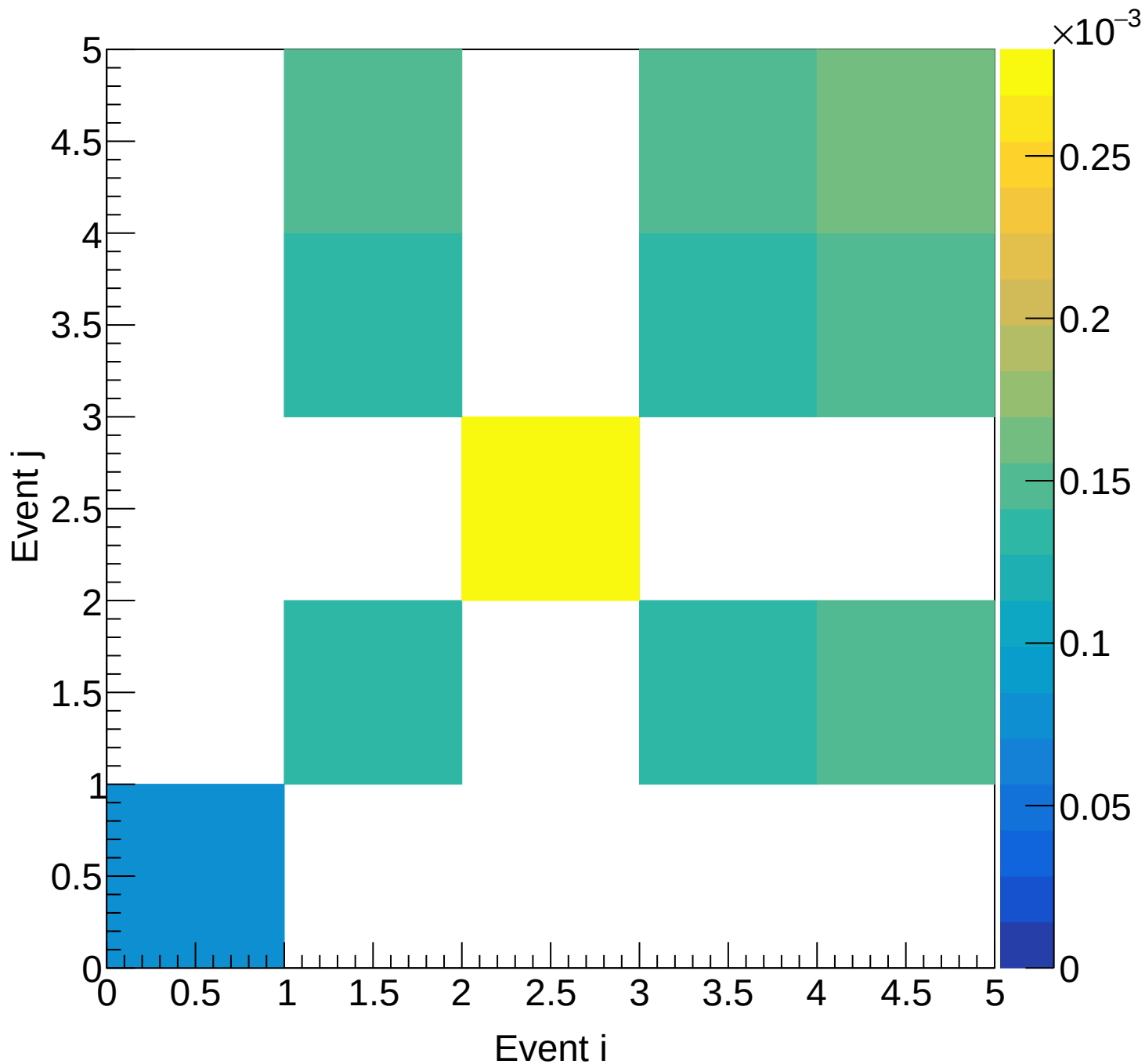
LD2 (total) Covariance | M: [7.5, 8.8) xF: [0.40, 0.45)
