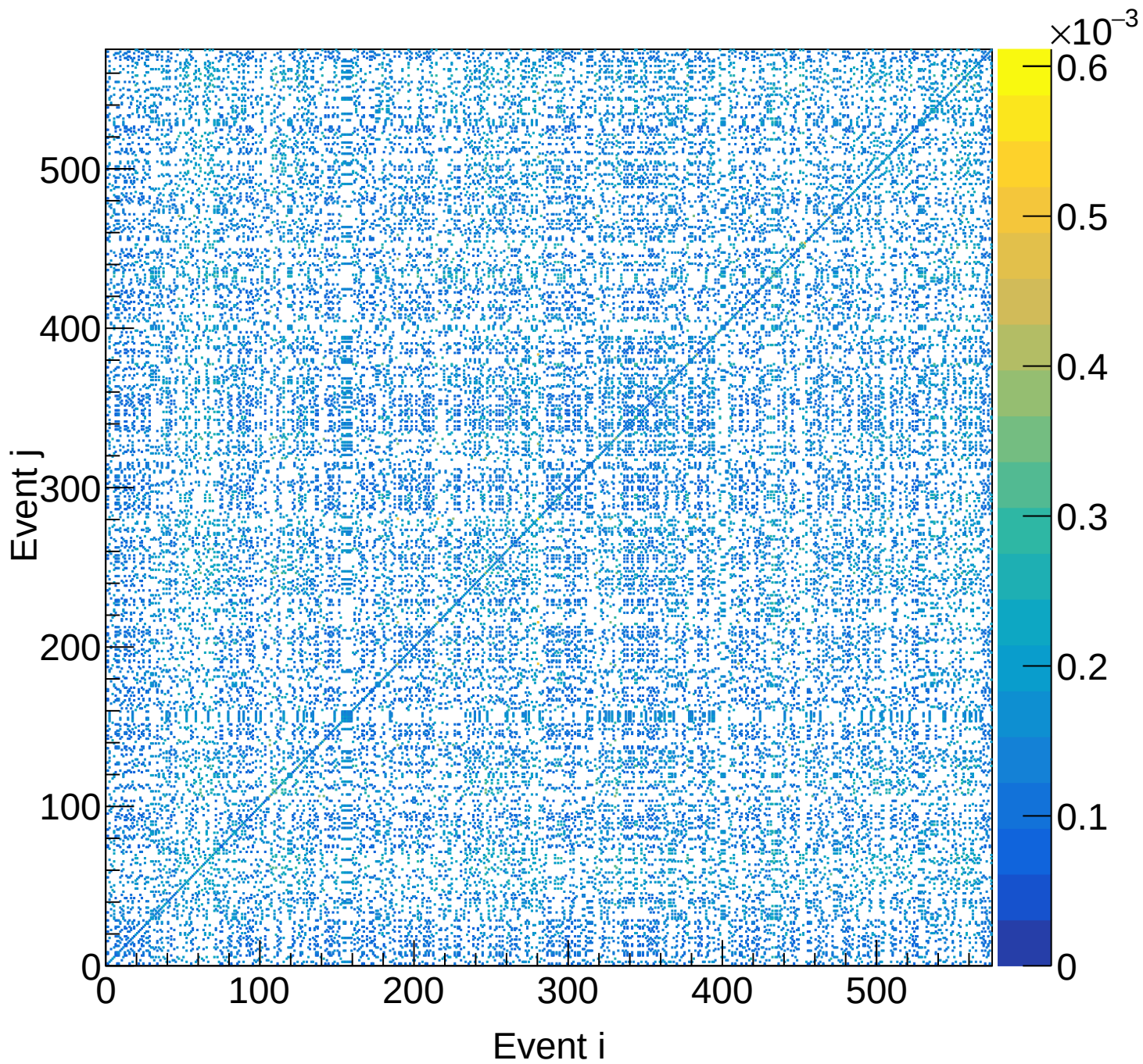
LD2 (total) Covariance | M: [4.5, 4.8) xF: [0.40, 0.45)
