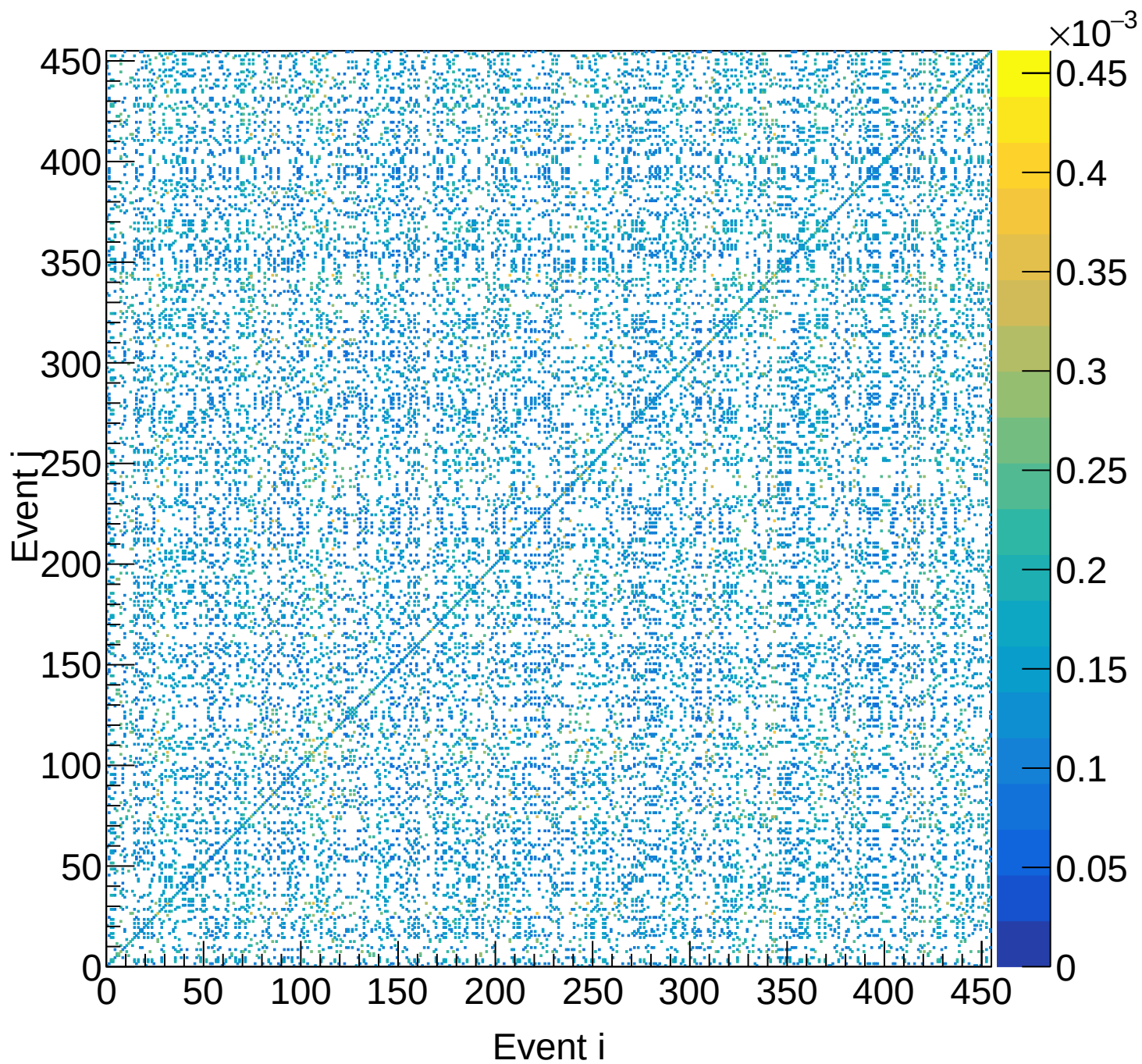
LD2 (total) Covariance | M: [4.8, 5.1) xF: [0.40, 0.45)
