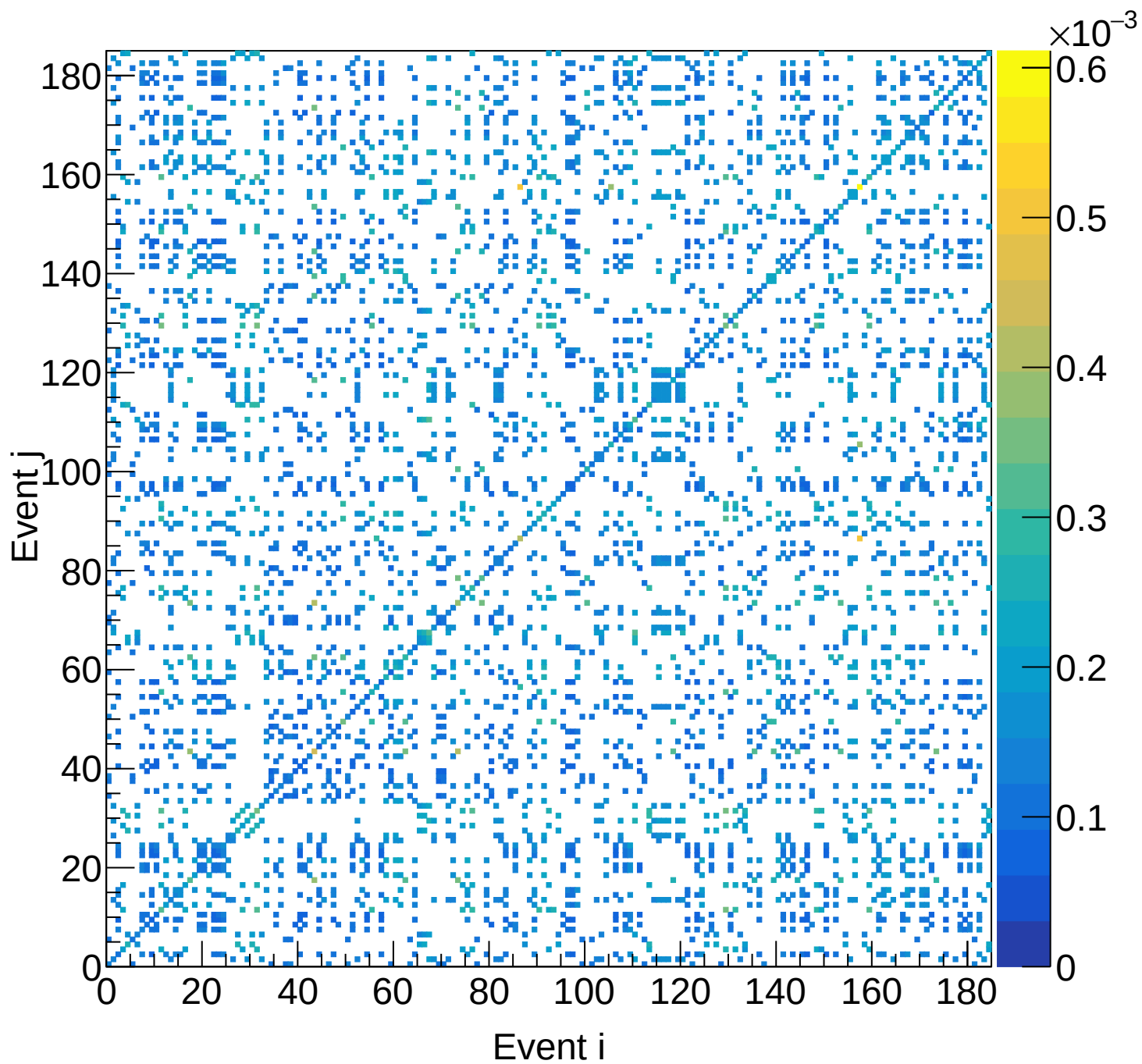
LD2 (total) Covariance | M: [5.4, 5.7) xF: [0.40, 0.45)
