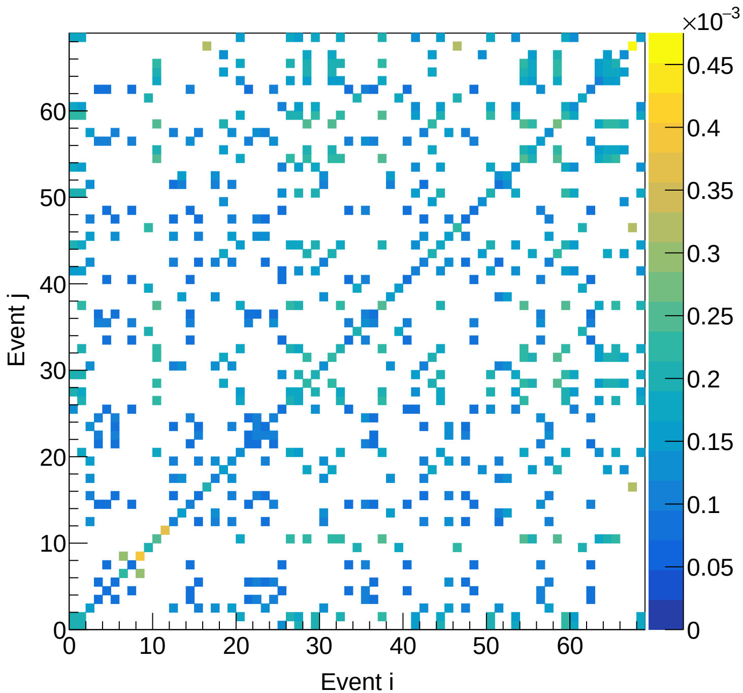
LD2 (total) Covariance | M: [6.0, 6.3] xF: [0.40, 0.45]
