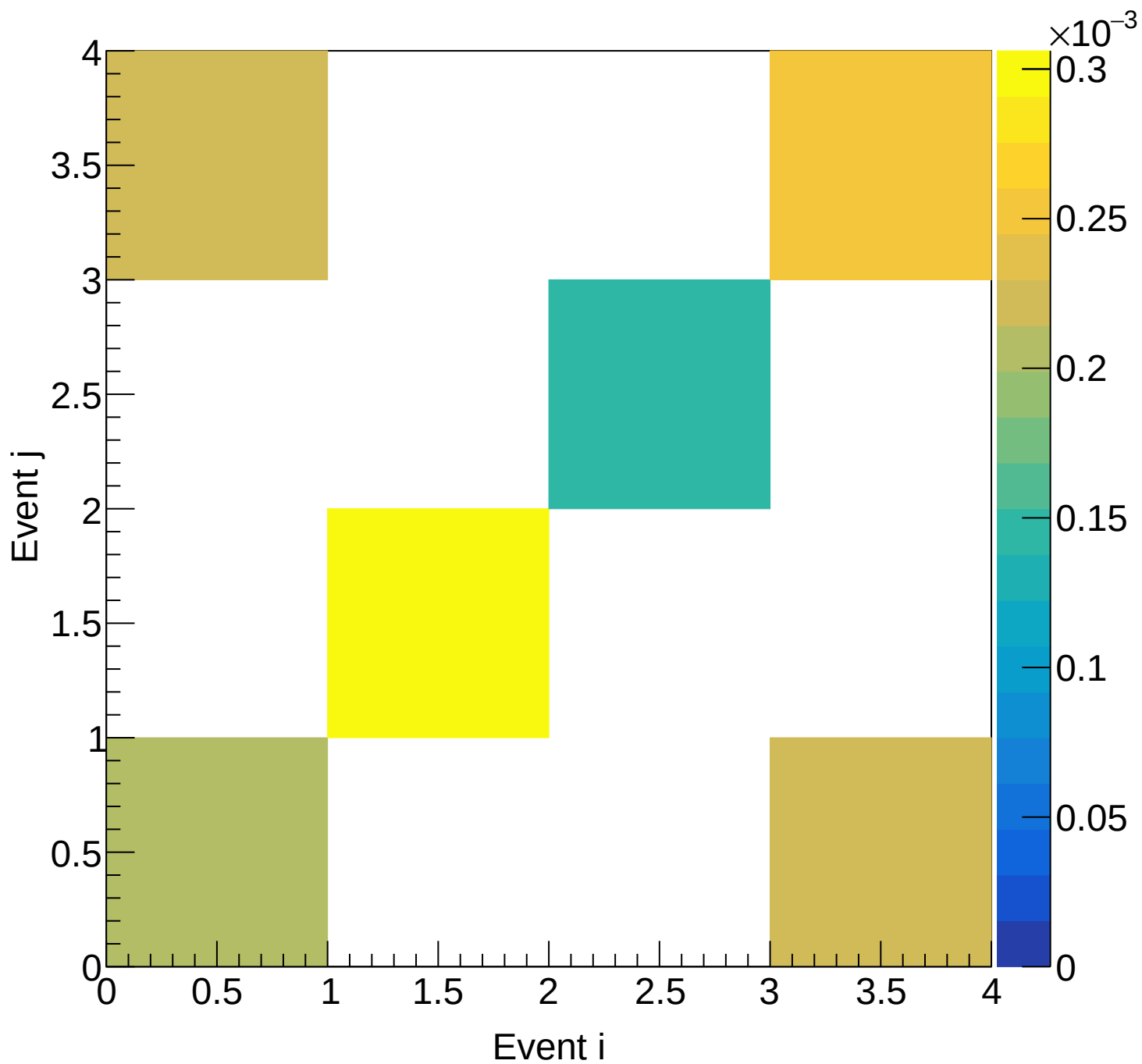
LH2 (mix) Covariance | M: [4.8, 5.1] xF: [-0.05, 0.00)
