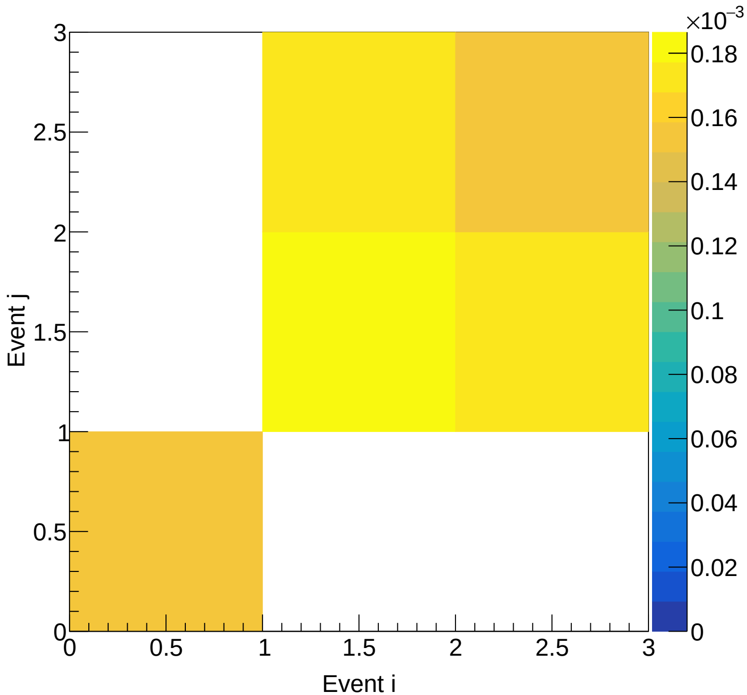
LH2 (mix) Covariance | M: [5.1, 5.4] xF: [-0.05, 0.00]
