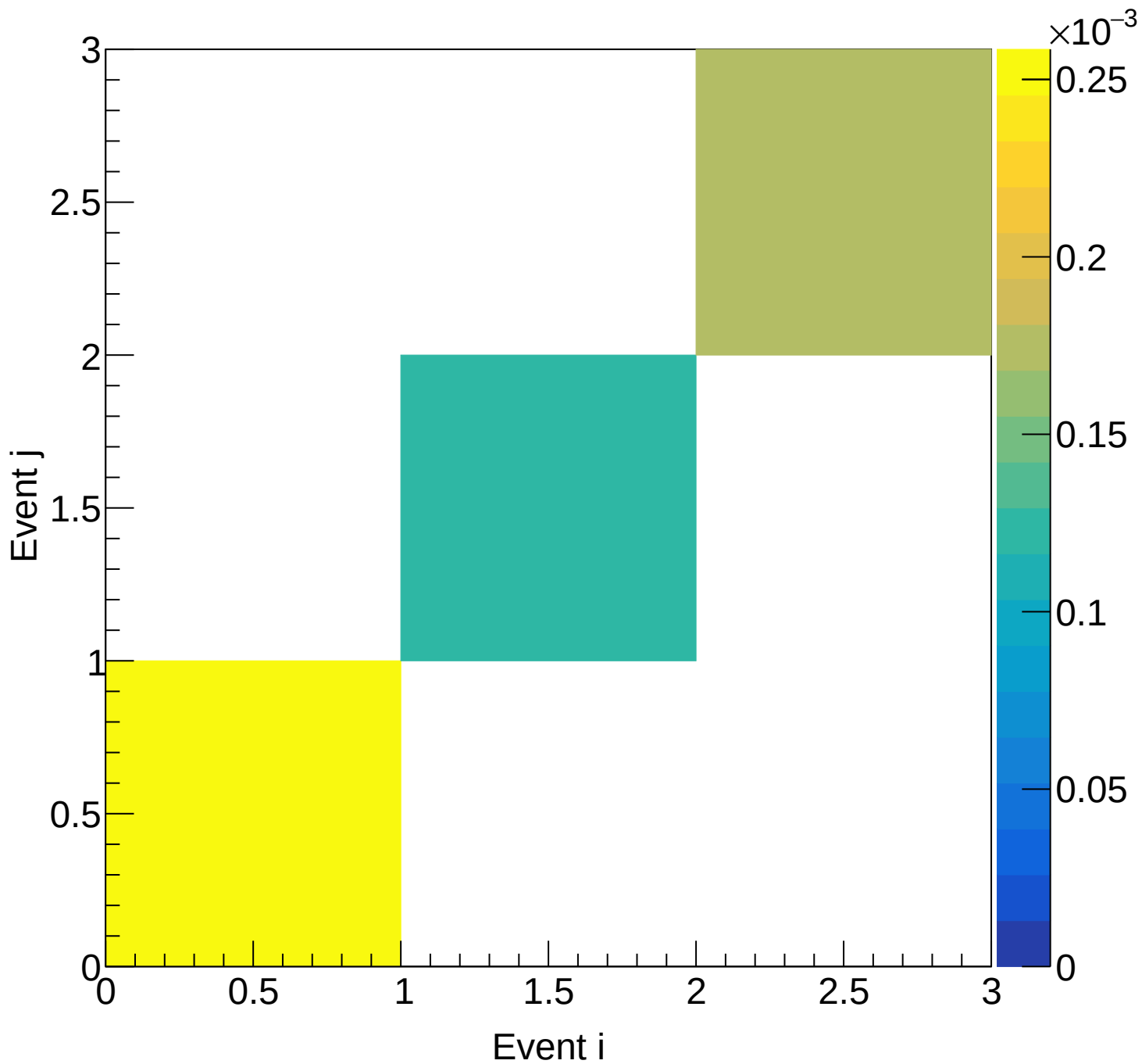
LH2 (mix) Covariance | M: [5.7, 6.0] xF: [-0.05, 0.00)
