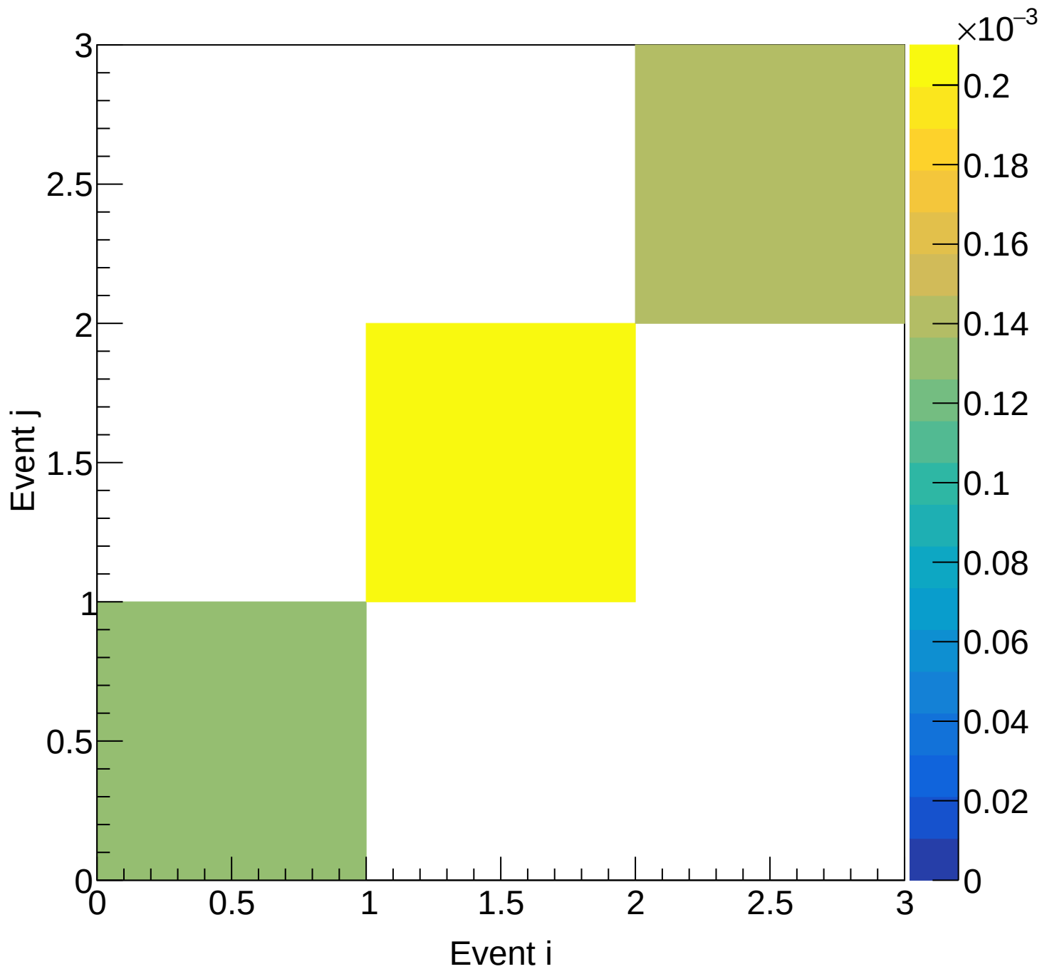
LH2 (mix) Covariance | M: [6.0, 6.3] xF: [-0.05, 0.00]
