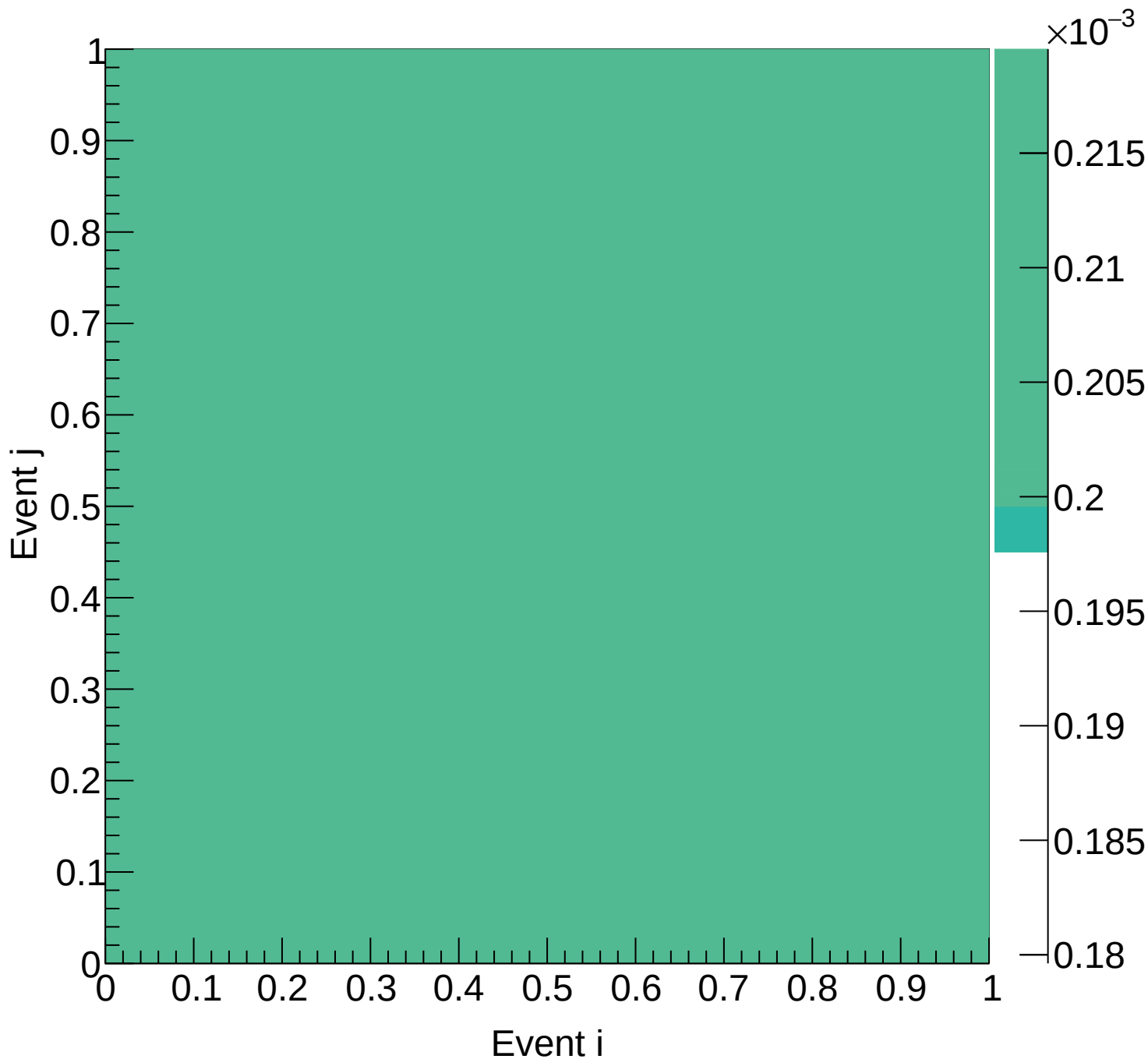
LH2 (mix) Covariance | M: [6.3, 6.6] xF: [-0.05, 0.00)
