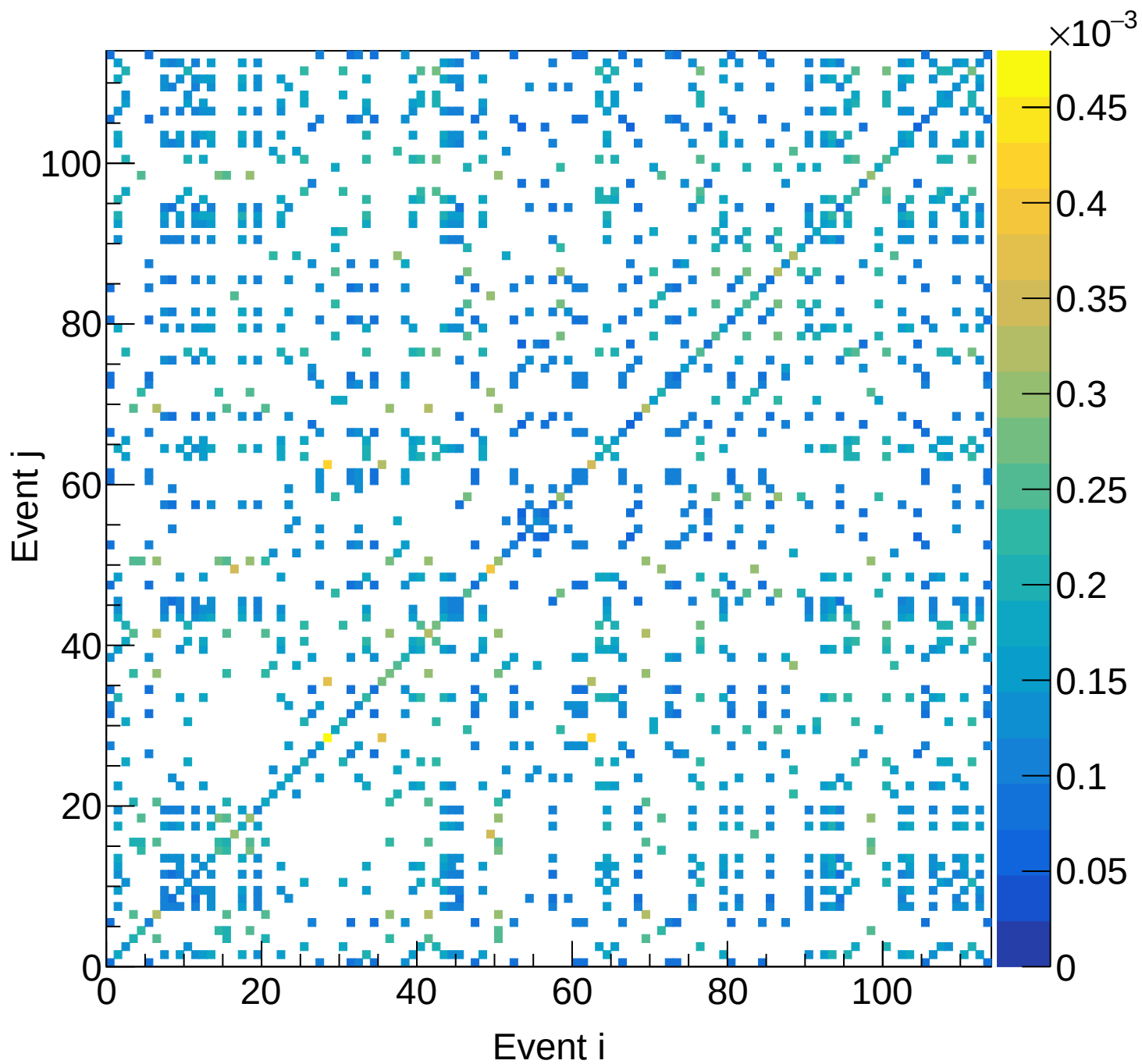
LH2 (mix) Covariance | M: [3.9, 4.2] xF: [0.45, 0.50)
