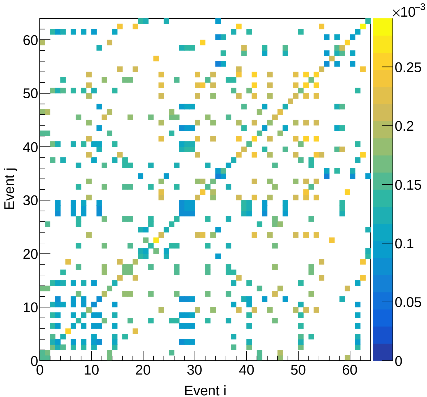
LH2 (mix) Covariance | M: [4.2, 4.5) xF: [0.45, 0.50)
