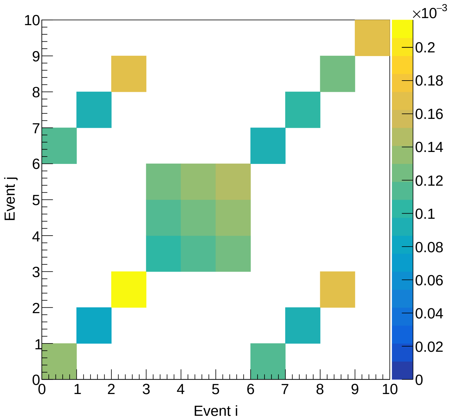
LH2 (mix) Covariance | M: [4.8, 5.1] xF: [0.45, 0.50]
