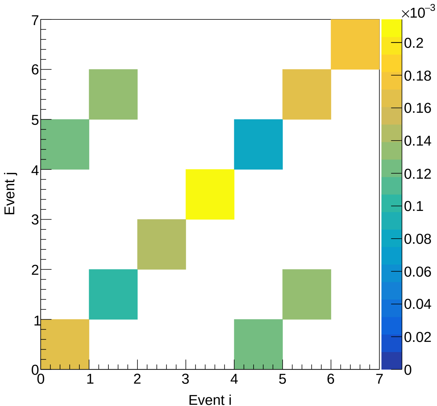
LH2 (mix) Covariance | M: [5.1, 5.4) xF: [0.45, 0.50)
