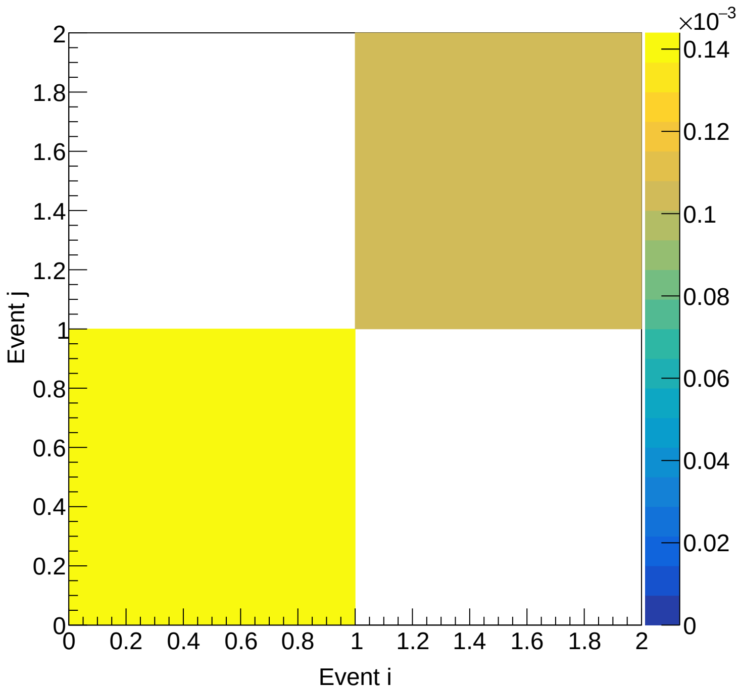
LH2 (mix) Covariance | M: [5.4, 5.7) xF: [0.45, 0.50)
