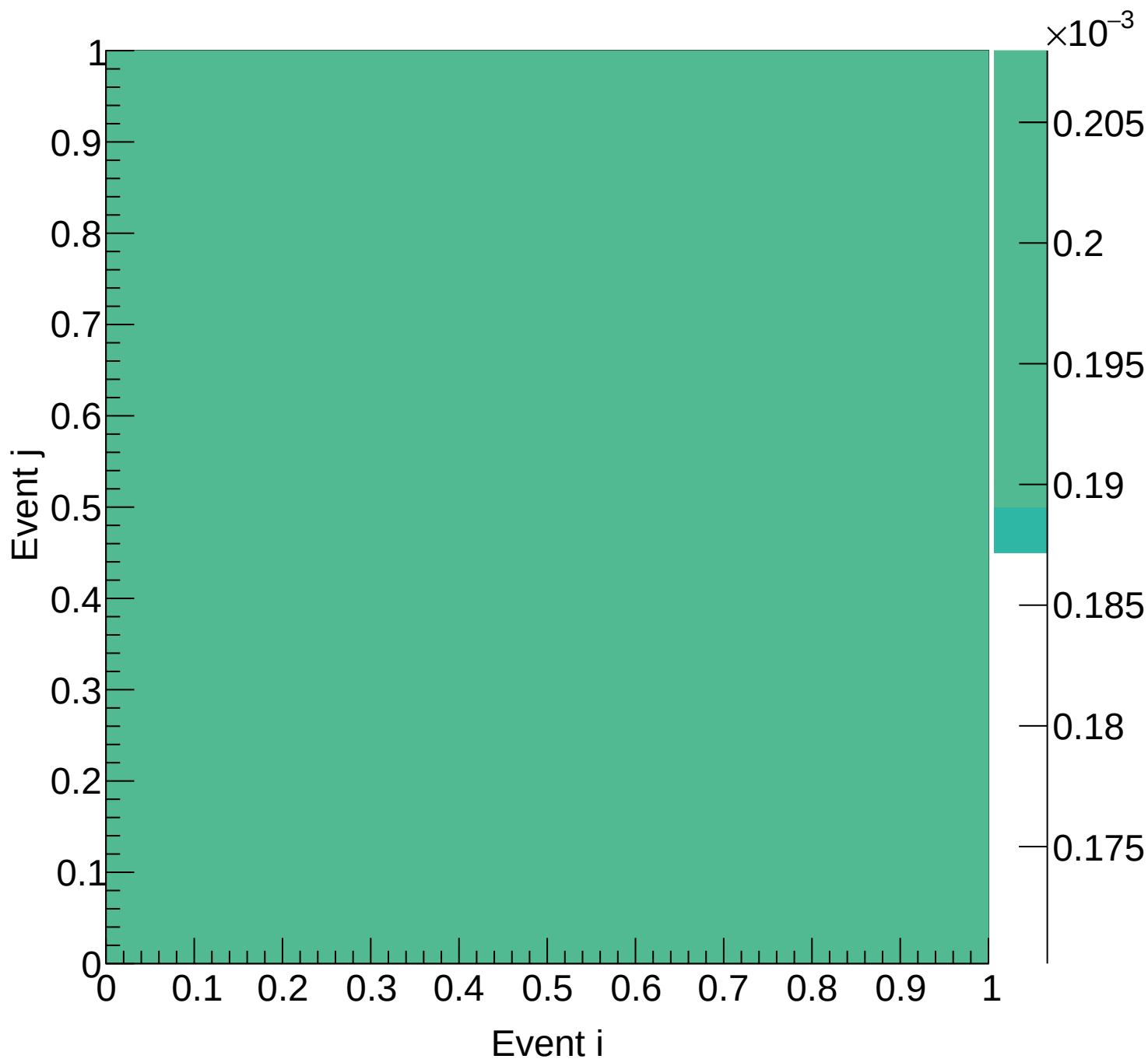
LH2 (mix) Covariance | M: [6.6, 6.9) xF: [0.45, 0.50)
