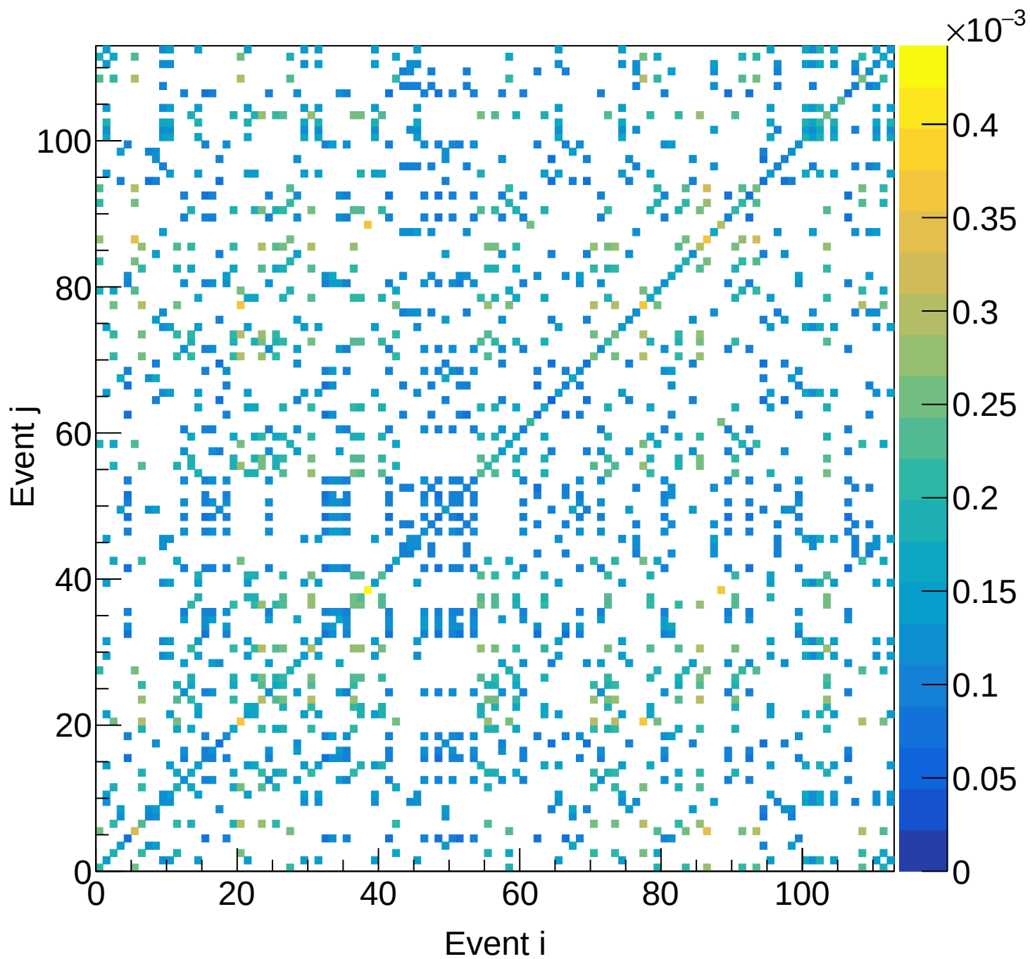
LH2 (mix) Covariance | M: [3.9, 4.2) xF: [0.50, 0.55)
