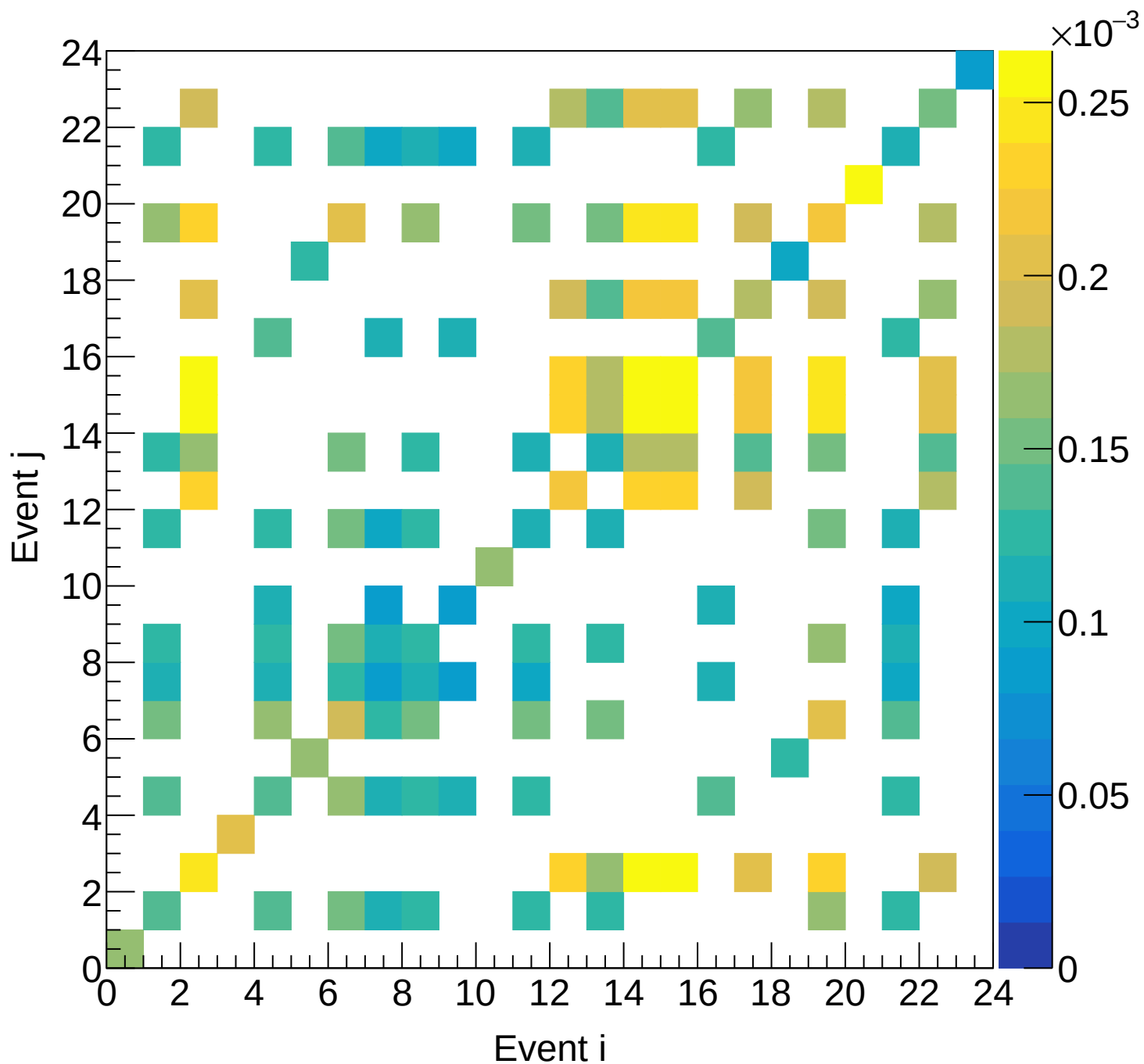
LH2 (mix) Covariance | M: [4.5, 4.8) xF: [0.50, 0.55)
