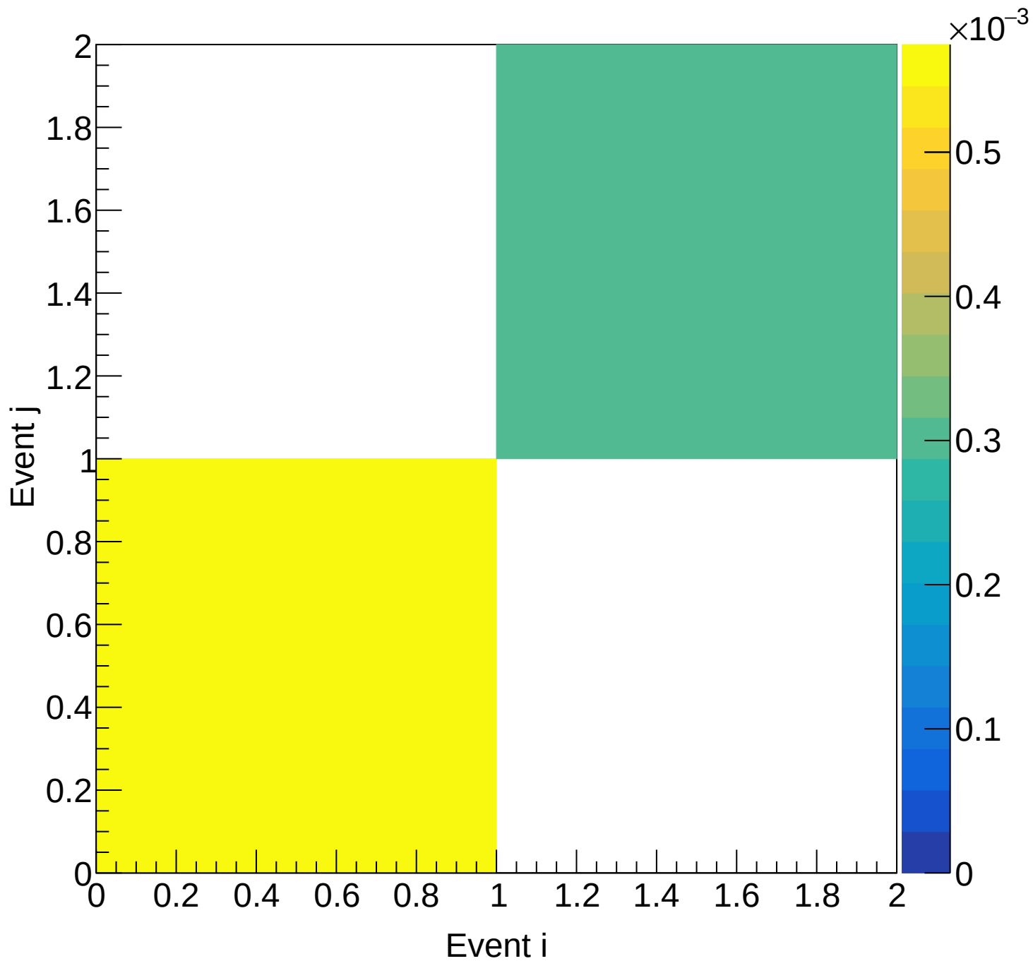
LH2 (mix) Covariance | M: [5.4, 5.7] xF: [0.50, 0.55]
