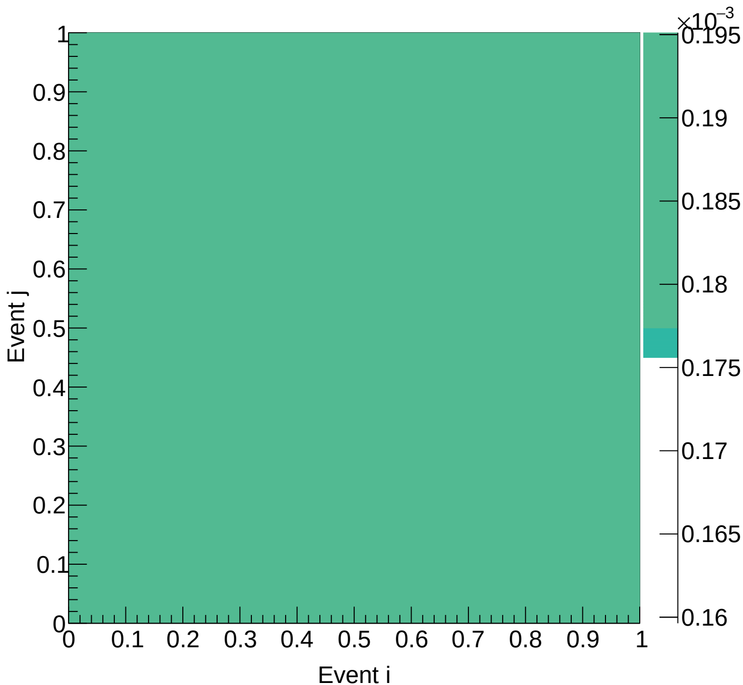
LH2 (mix) Covariance | M: [5.7, 6.0] xF: [0.50, 0.55)
