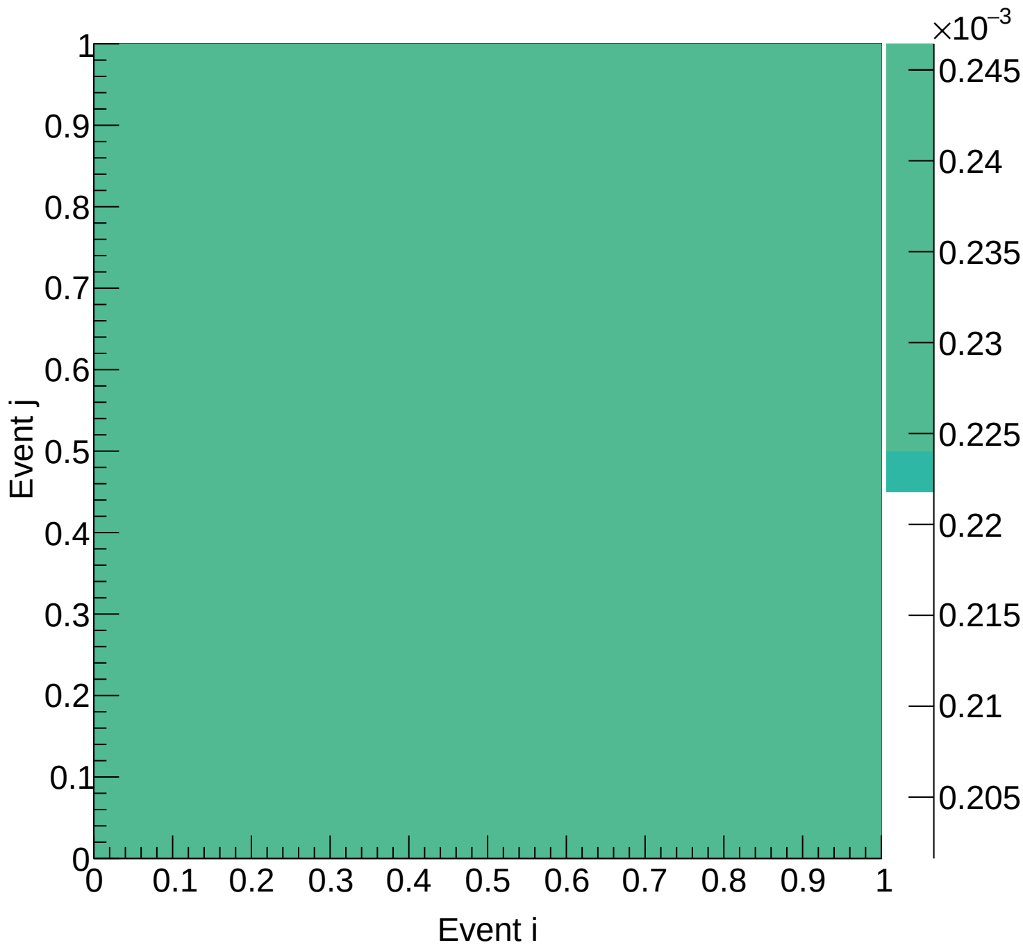
LH2 (mix) Covariance | M: [6.0, 6.3) xF: [0.50, 0.55)
