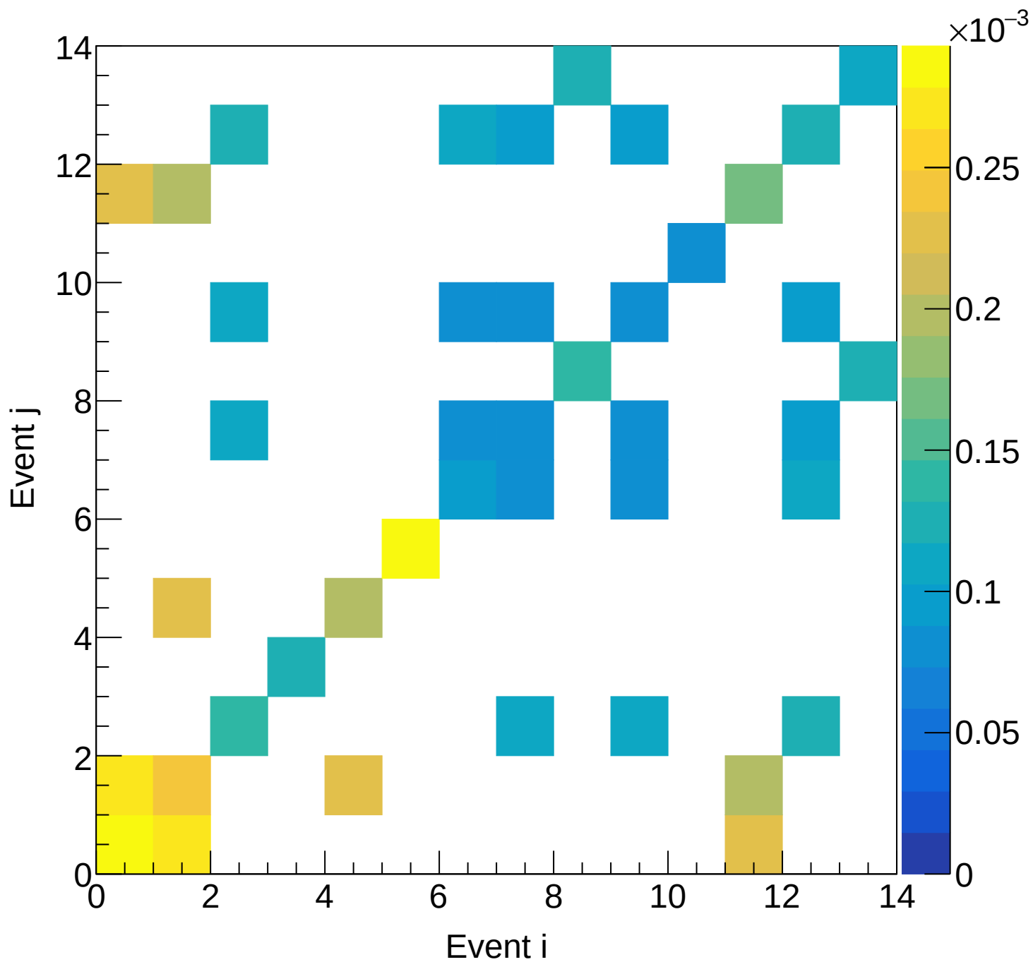
LH2 (mix) Covariance | M: [4.5, 4.8) xF: [0.55, 0.60)
