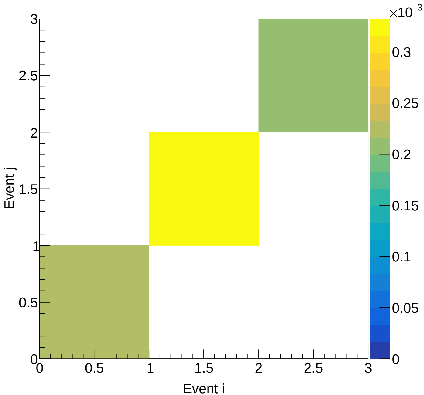
LH2 (mix) Covariance | M: [5.4, 5.7) xF: [0.55, 0.60)
