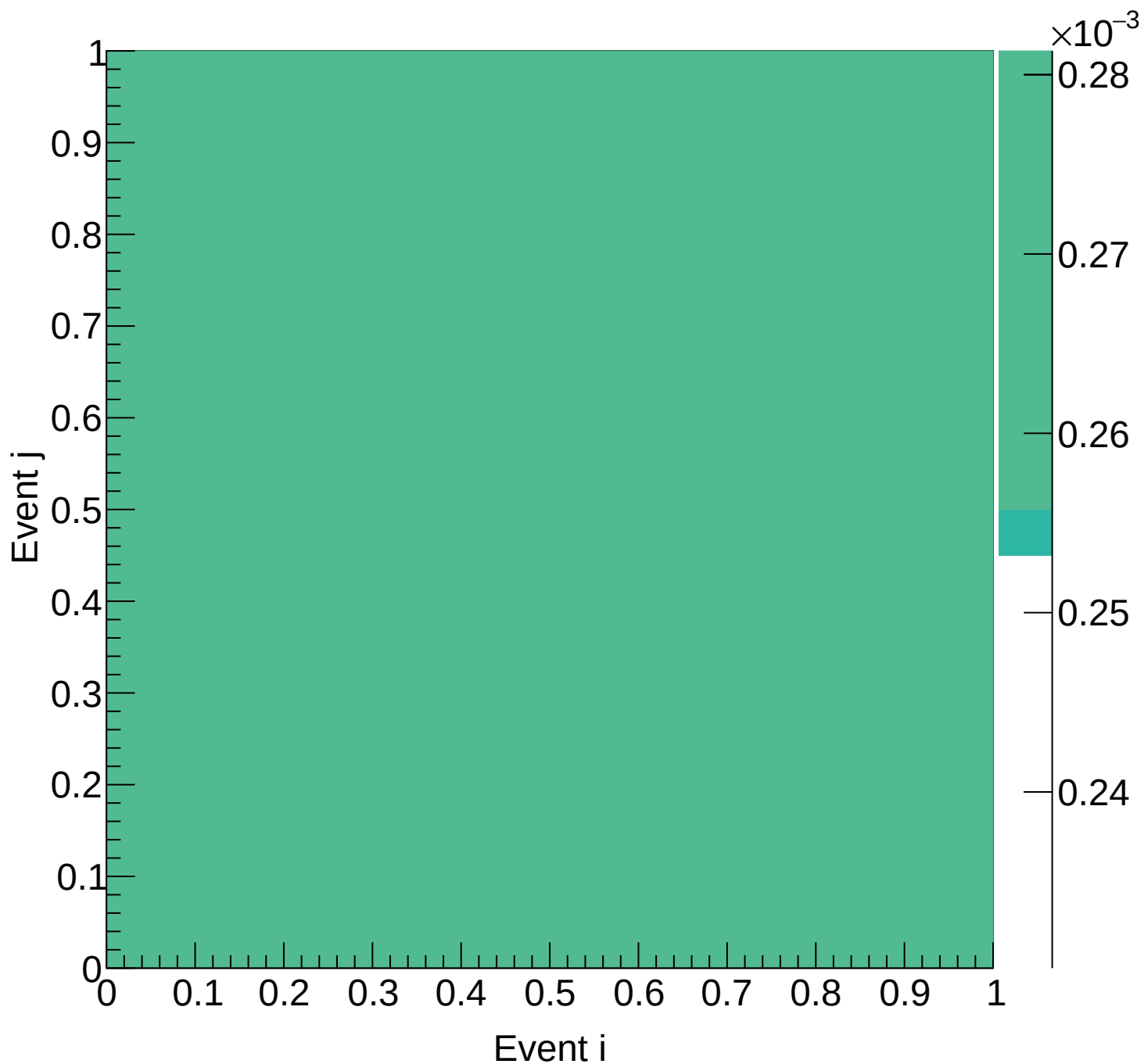
LH2 (mix) Covariance | M: [6.9, 7.5] xF: [0.60, 0.65)
