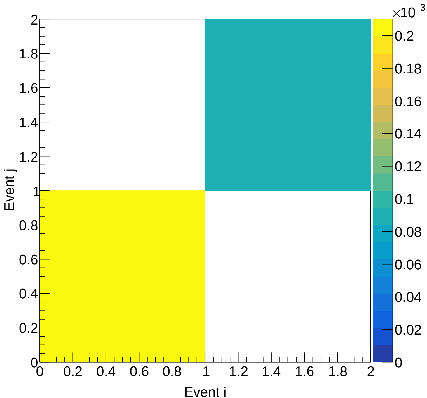
LH2 (mix) Covariance | M: [5.4, 5.7) xF: [0.60, 0.65)
