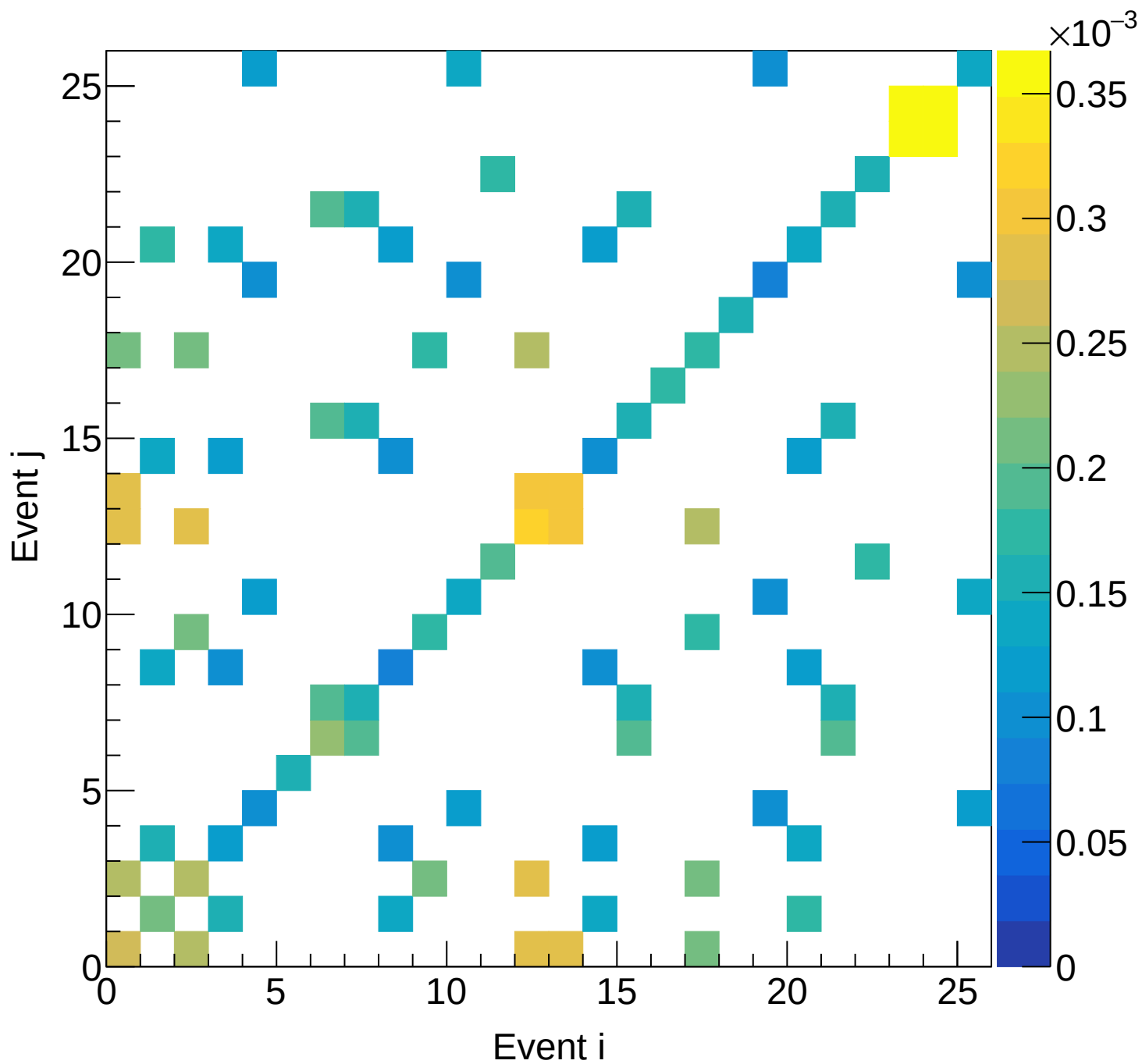
LH2 (mix) Covariance | M: [4.2, 4.5] xF: [0.65, 0.70)
