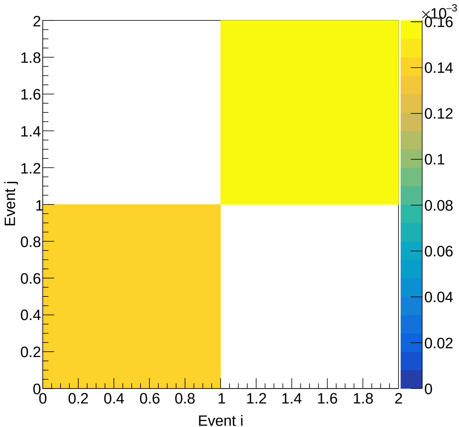
LH2 (mix) Covariance | M: [5.1, 5.4) xF: [0.65, 0.70)
