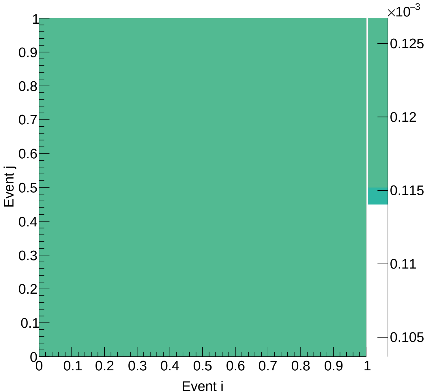
LH2 (mix) Covariance | M: [5.4, 5.7) xF: [0.65, 0.70)
