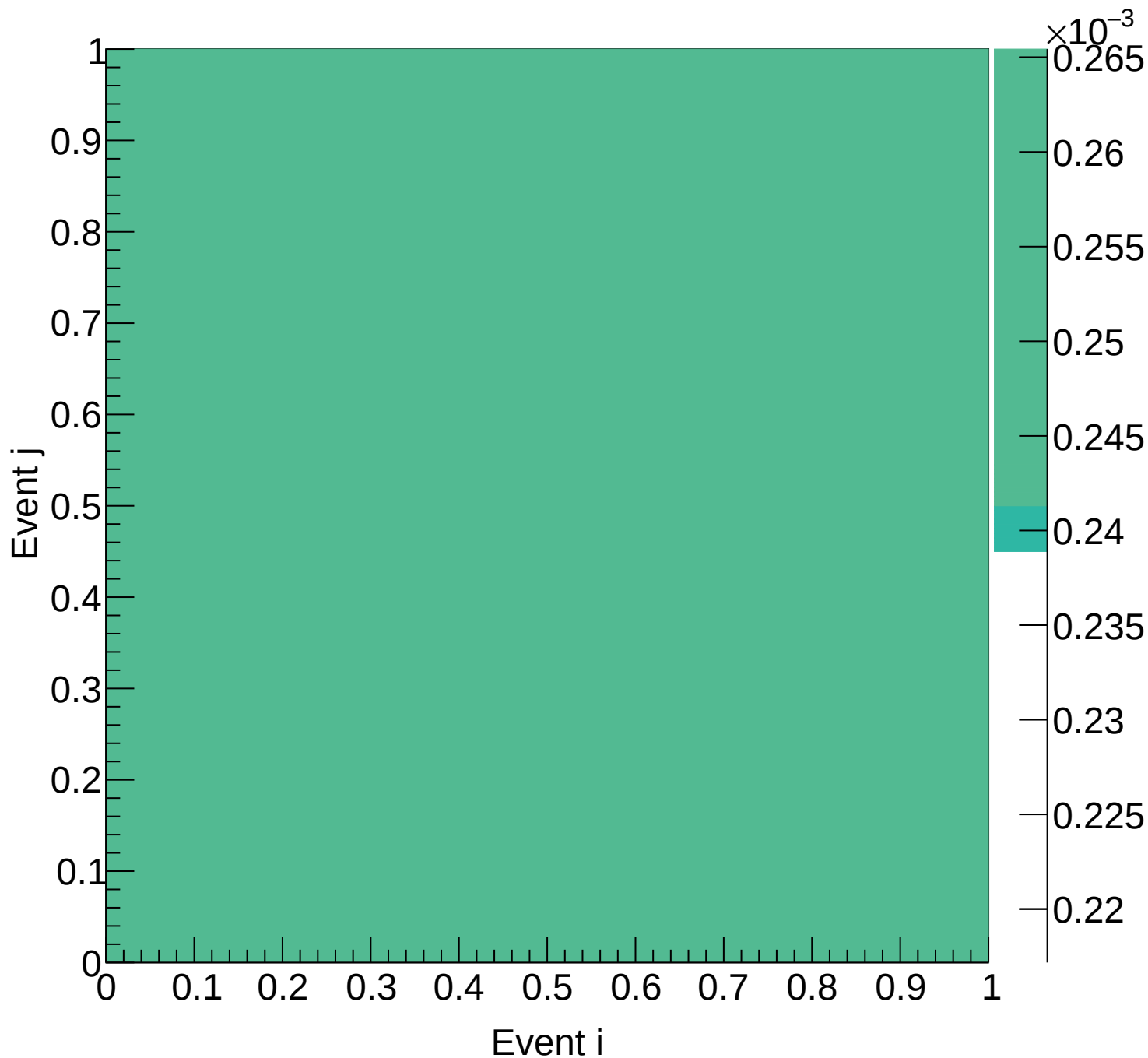
LH2 (mix) Covariance | M: [5.7, 6.0] xF: [0.65, 0.70)
