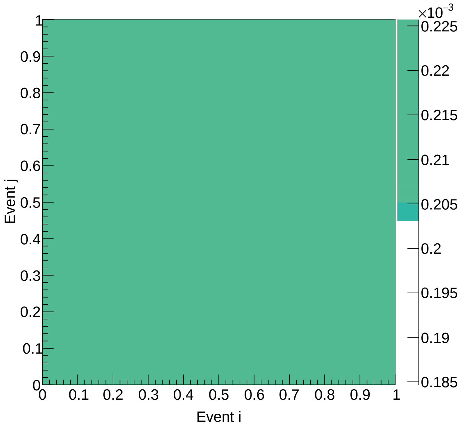
LH2 (mix) Covariance | M: [6.0, 6.3) xF: [0.65, 0.70)
