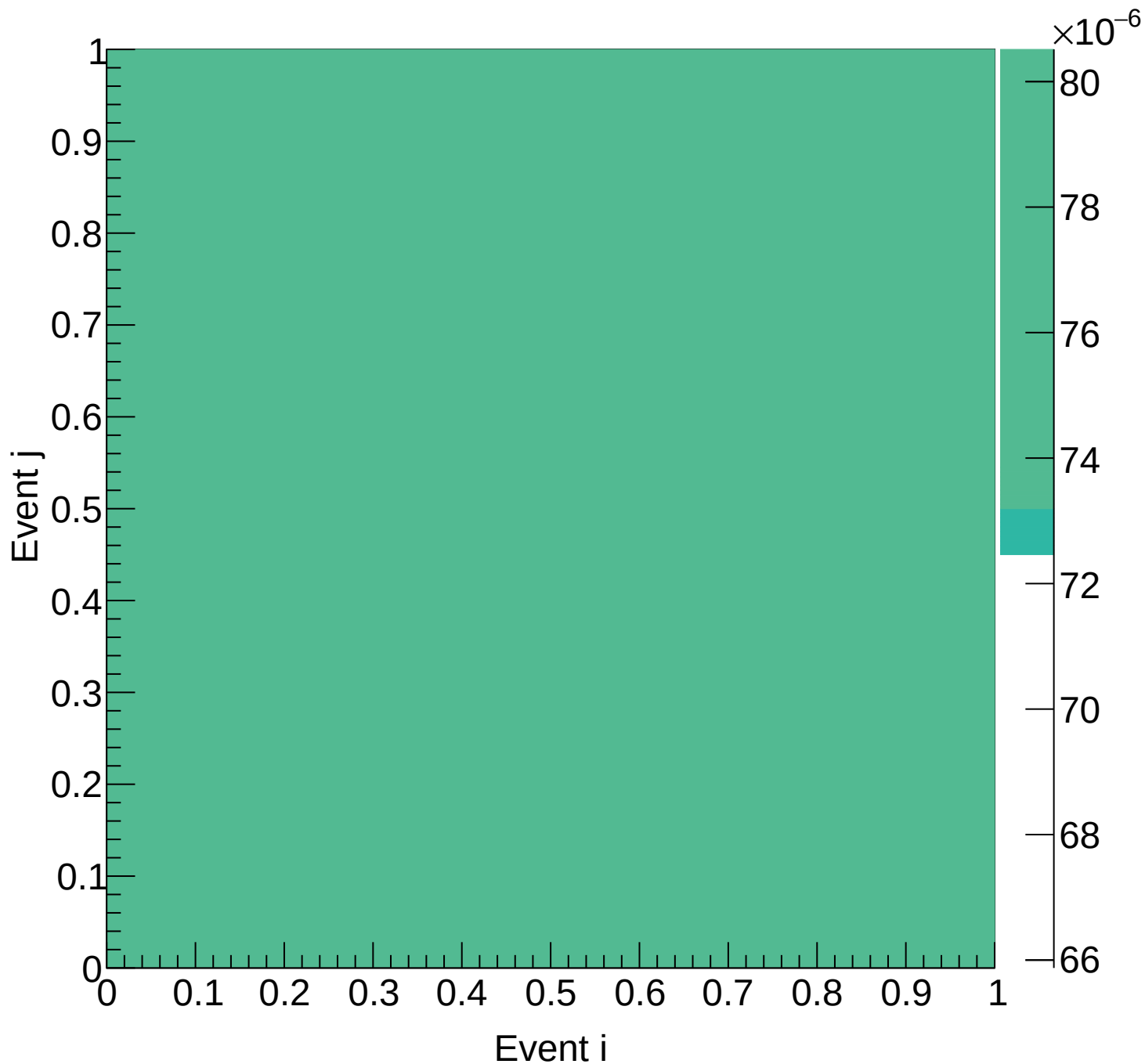
LH2 (mix) Covariance | M: [4.8, 5.1) xF: [0.70, 0.75)
